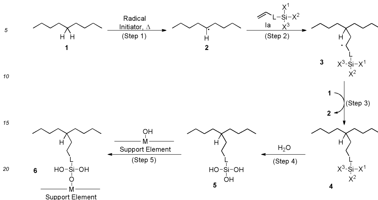
Scheme 1. Proposed Mechanism of Vinyl Silane Mediated Bonding Between Graft Material and Stent
