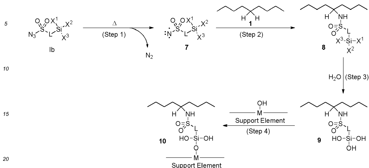
Scheme 2. Proposed Mechanism of Azidosulfonyl Silane Mediated Bonding Between Graft Material and Stent
