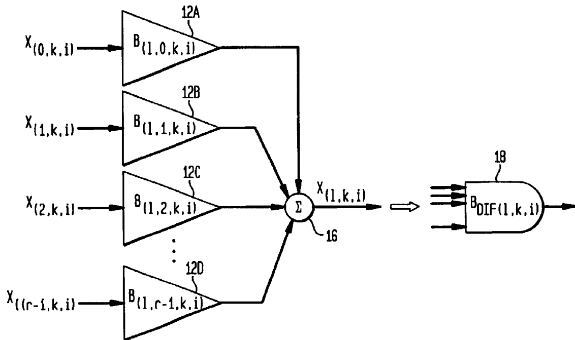
SIMPLIFIED JABER'S RADIX-r DIF ENGINE
