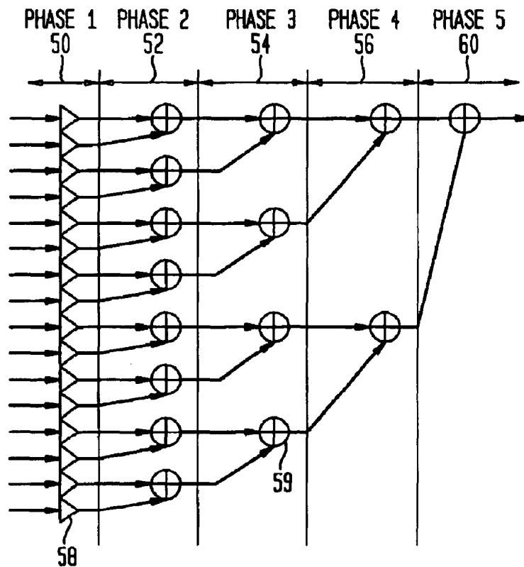
FIG. 6B RADIX-16 DIF FFT ENGINE
