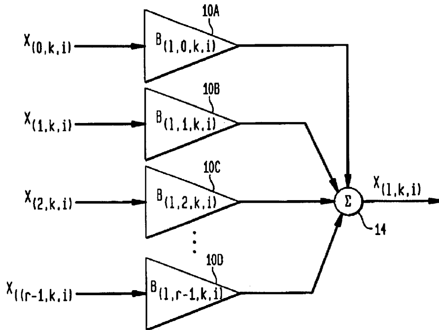
JABER'S RADIX-r DIF ENGINE
