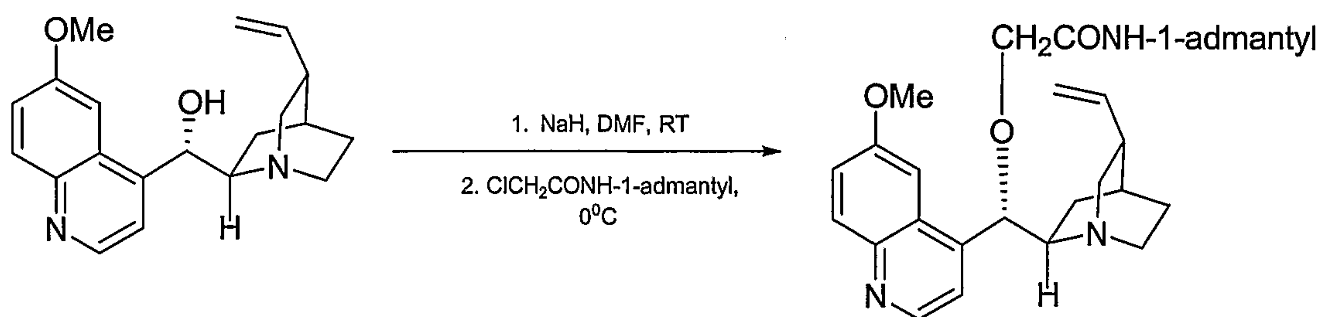
O-(1-adamantylacetamide)quinidine
