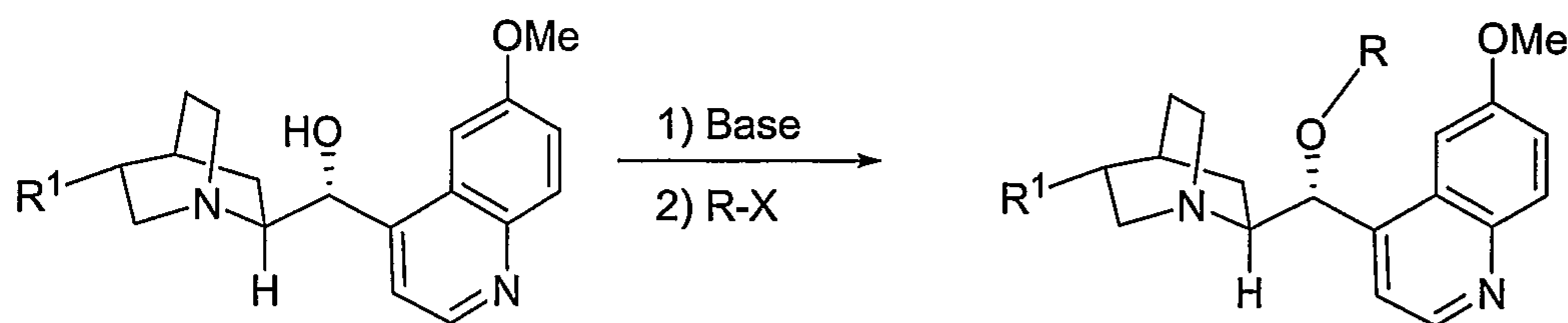
Scheme 2
