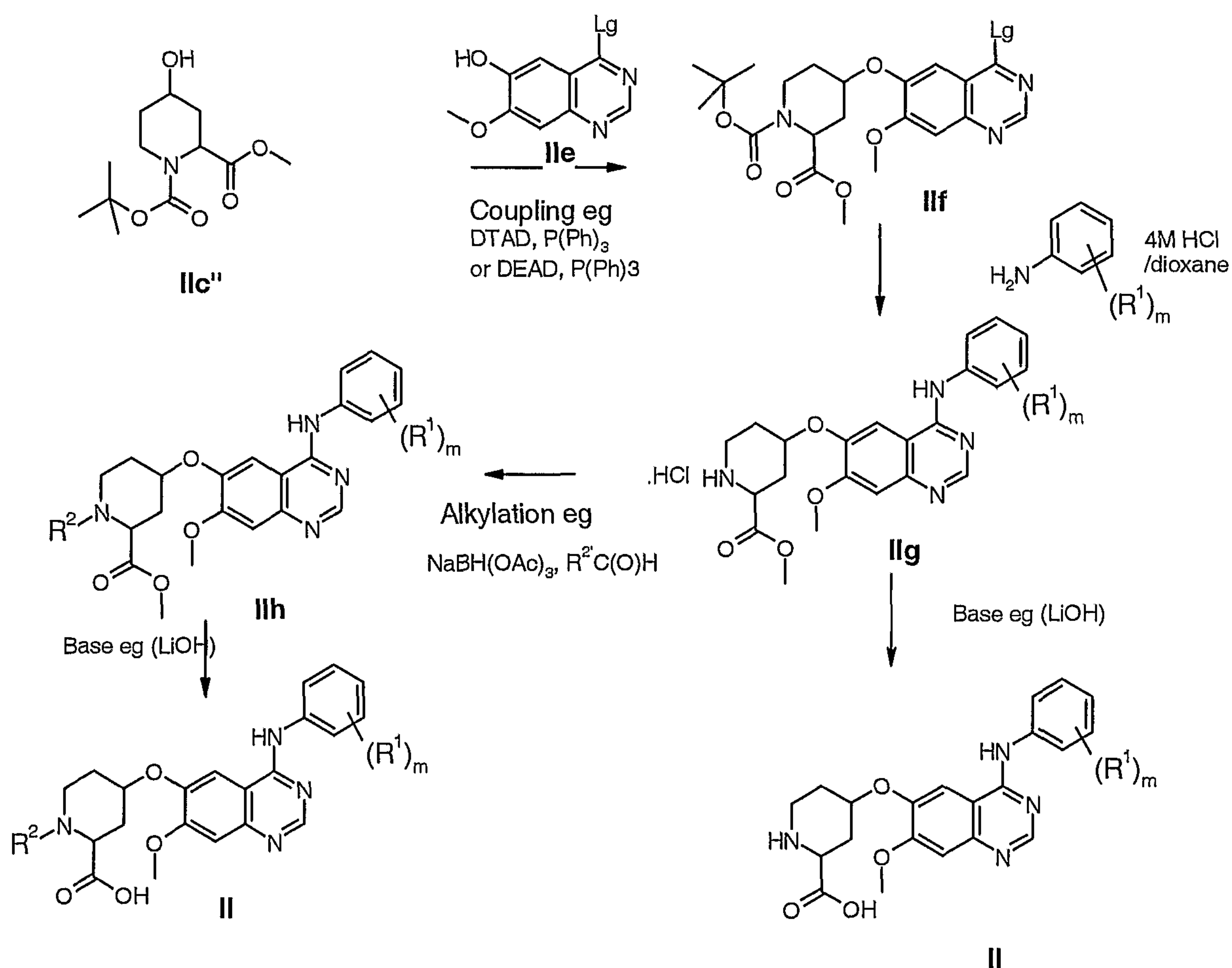
Reaction Scheme Ia:
