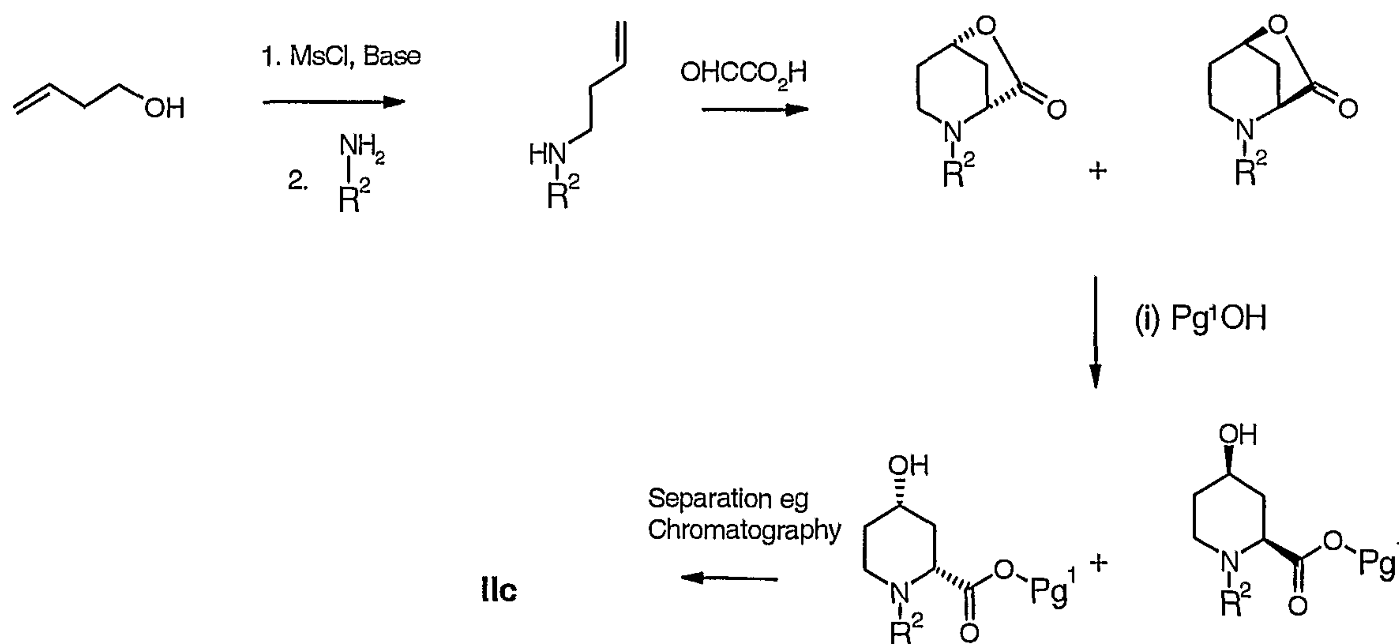
Reaction Scheme 2b
