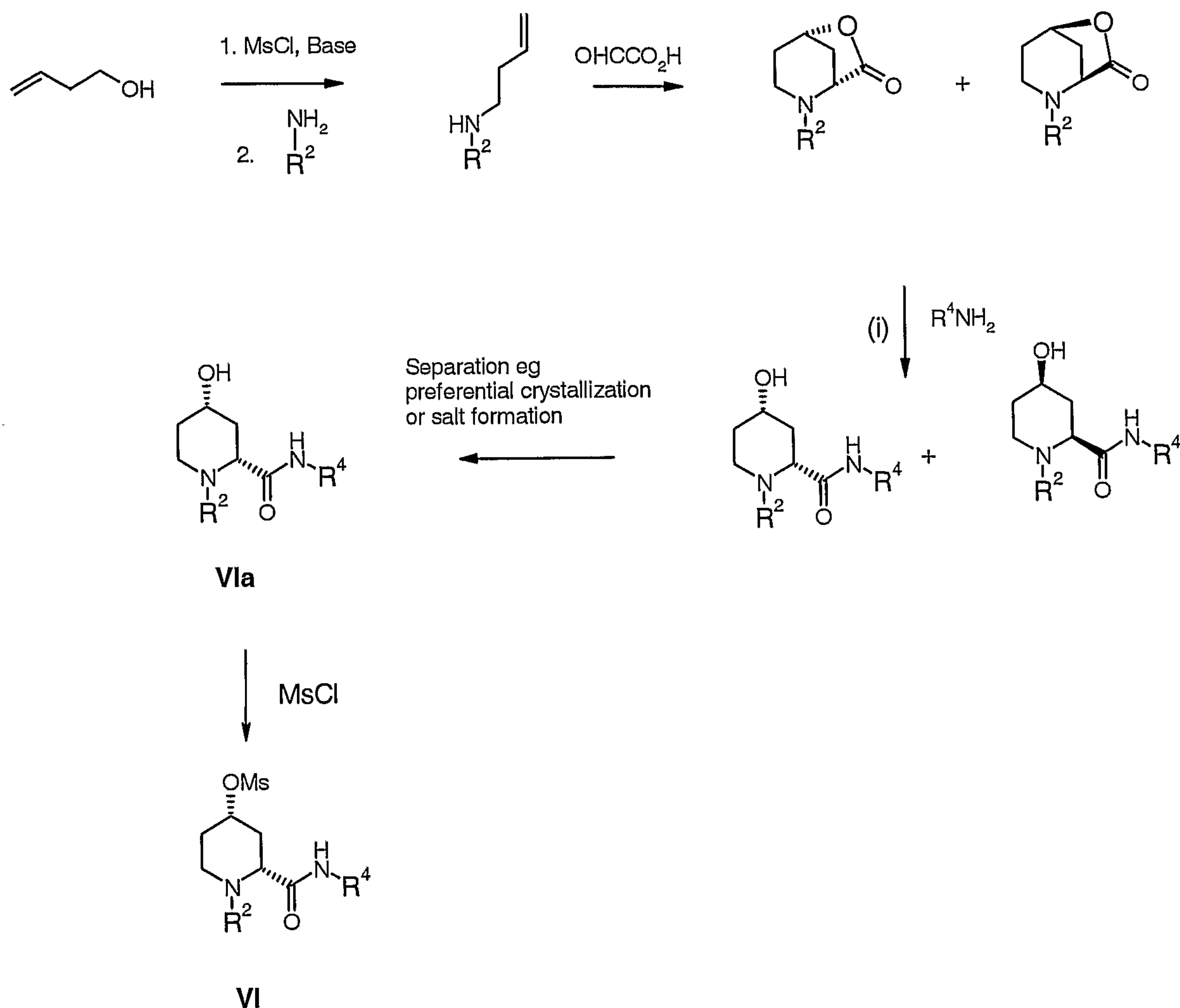
Reaction Scheme 4a
