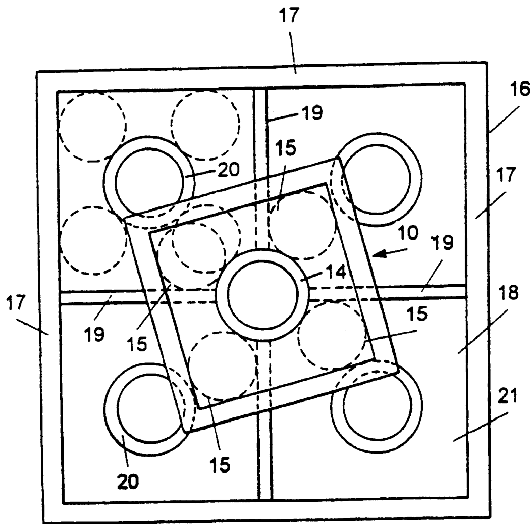
Fig. 3 PRIOR ART
