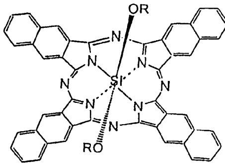
Silicon Naphthalocyanine
