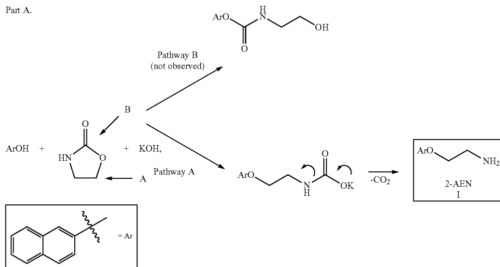
Scheme 1. Proposed mechanism of the synthesis of 2-AEN and by-products
