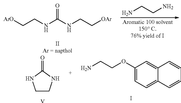
Scheme 2. Conversion of N,N'-bis(2-(2-naphthoxy)ethyl) Urea to 2-AEN
