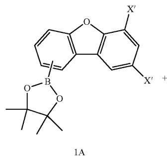
[Reaction Scheme 1]
