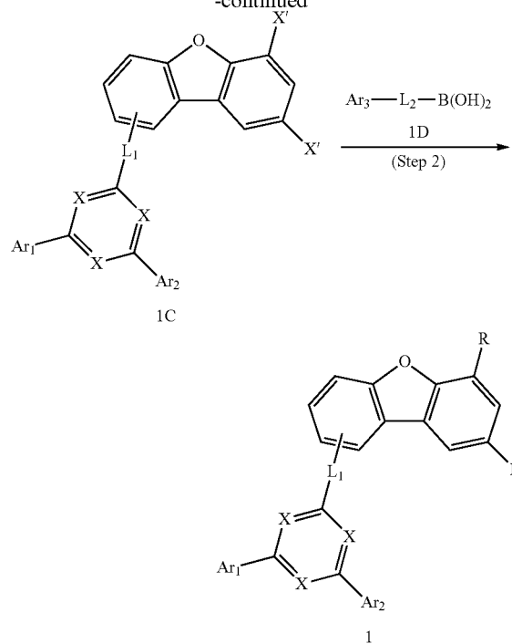
[Reaction Scheme 2]
