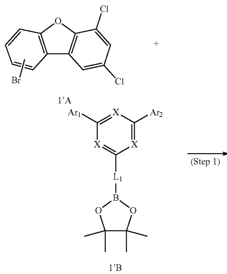
[Reaction Scheme 2]
