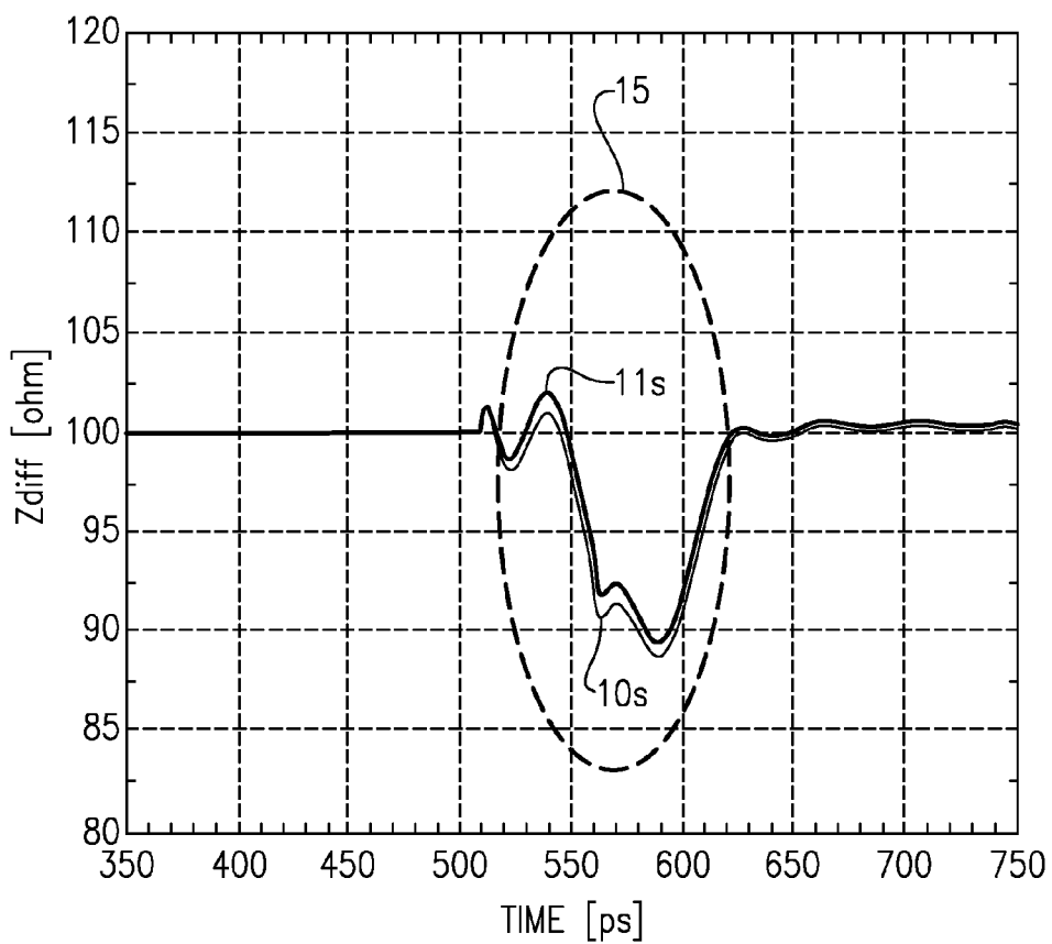
FIG.2 Prior Art
