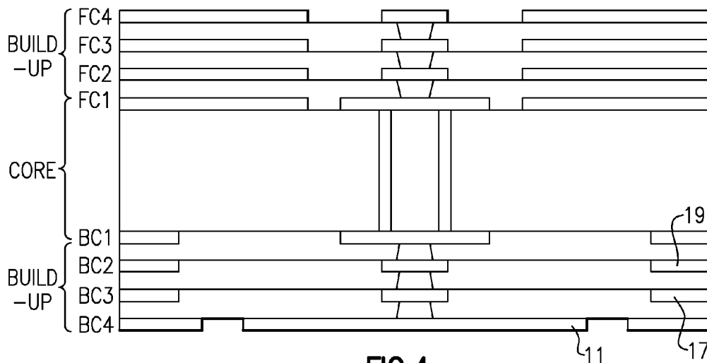
FIG.4 Prior Art
