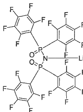
Chemical Formula: C_{24}F_{20}LiNO_2P_2 Molecular Weight: 783,12
