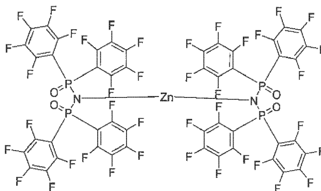
Chemical Formula: C_{48}F_{40}N_2O_4P_4Zn Molecular Weight: 1617,75
