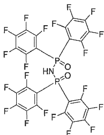
Chemical Formula: C_{24}HF_{20}NO_2P_2 Molecular Weight: 777,19
