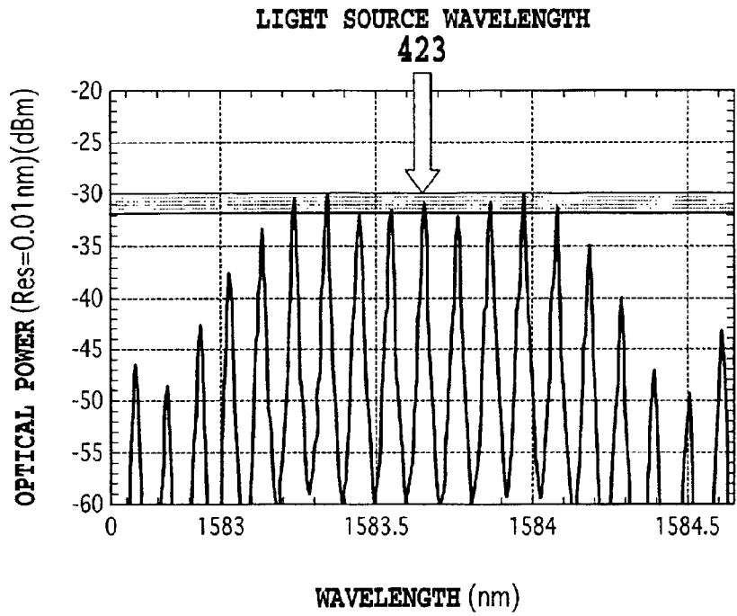
ODD-NUMBER-TH LIGHT SOURCE WAVELENGTH AND SIDE MODES
