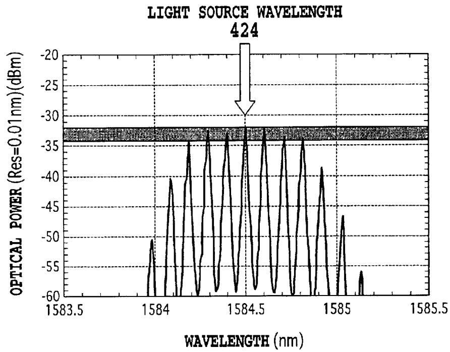
EVEN-NUMBER-TH LIGHT SOURCE WAVELENGTH AND SIDE MODES
