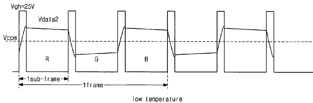
FIG. 3B Related Art
