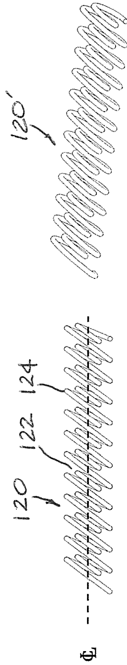
Canted Coil Spring - Variable Coil Dimensions
