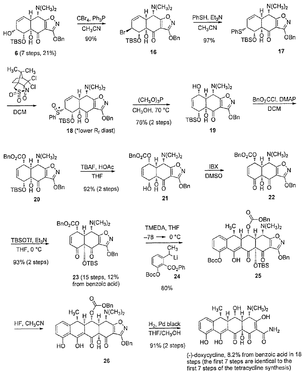
Figure 3 Total Synthesis of Doxycycline
