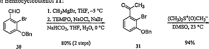
Figure 5 Synthesis of Benzocyclobutenol 11:
