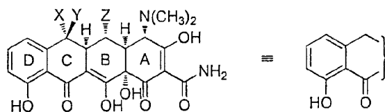
Figure 14A Representative Structures
