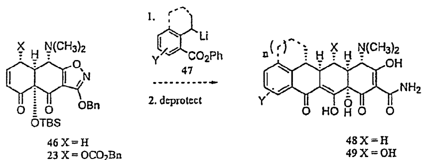
Figure 9 Summary of Targeted "Bridged-Pentacyclines"
