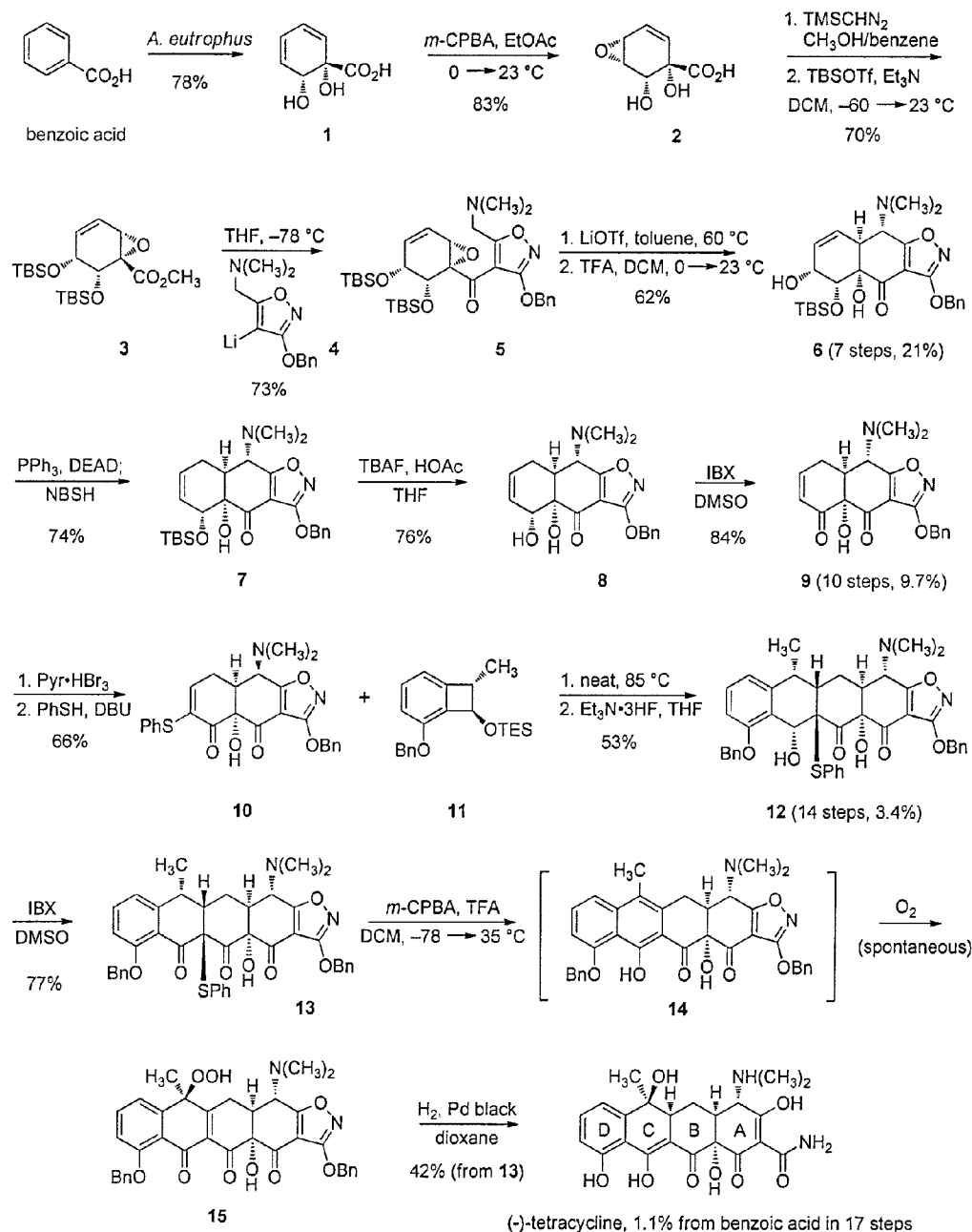
Figure 2 Total Synthesis of Tetracycline
