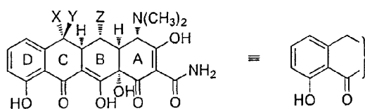
Figure 14B Representative Structures
