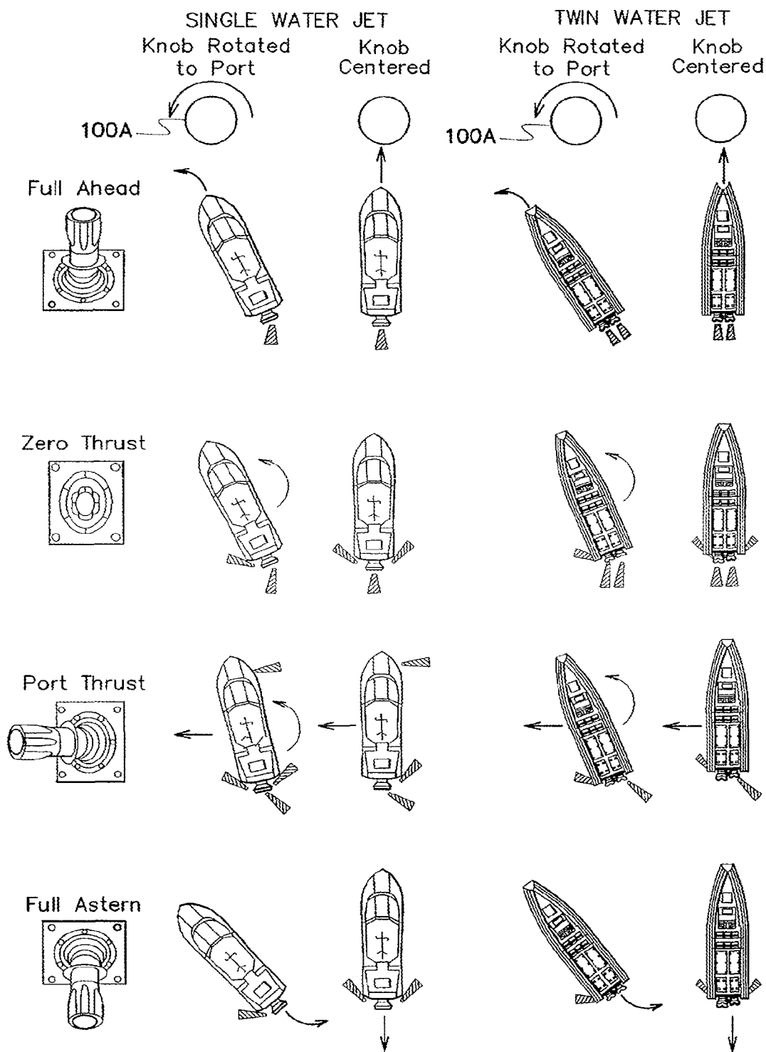
Three-Axis Joystick Implementation
