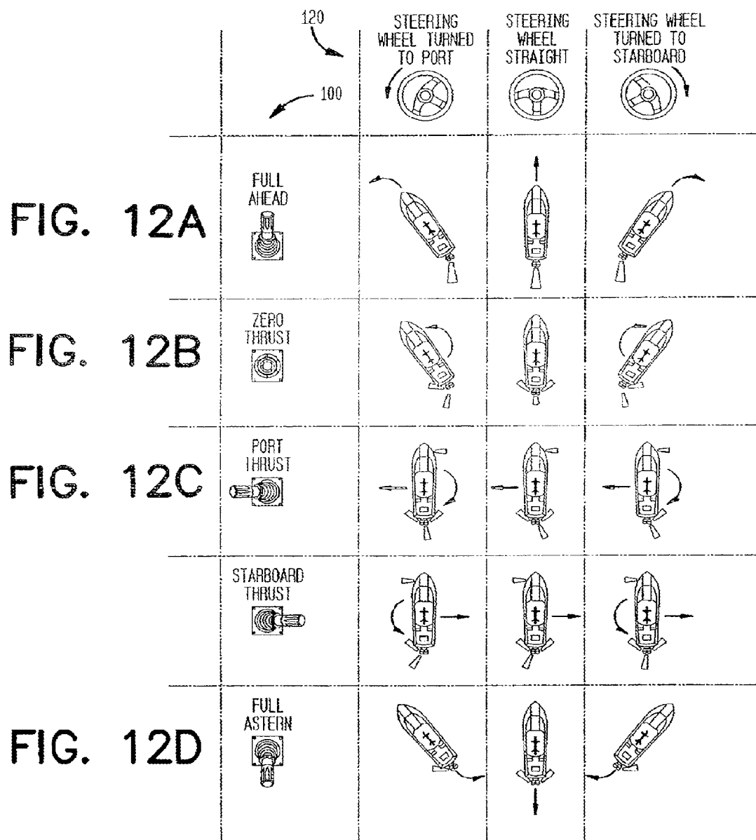
SINGLE WATERJET MOTION DIAGRAM
