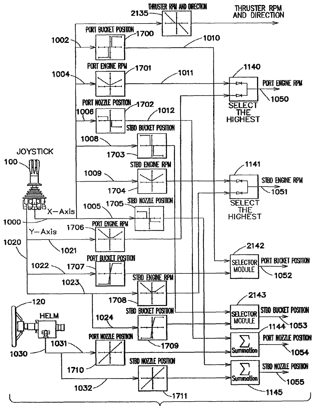
TWIN WATERJET SIGNAL DIAGRAM WITH BOWTHRUSTER
