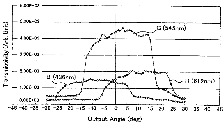
(a) DISTRIBUTION OF RGB EMITTED LIGHT FROM LIQUID CRYSTAL CELL (WITHOUT MICROPRISM BUILT IN CELL)
