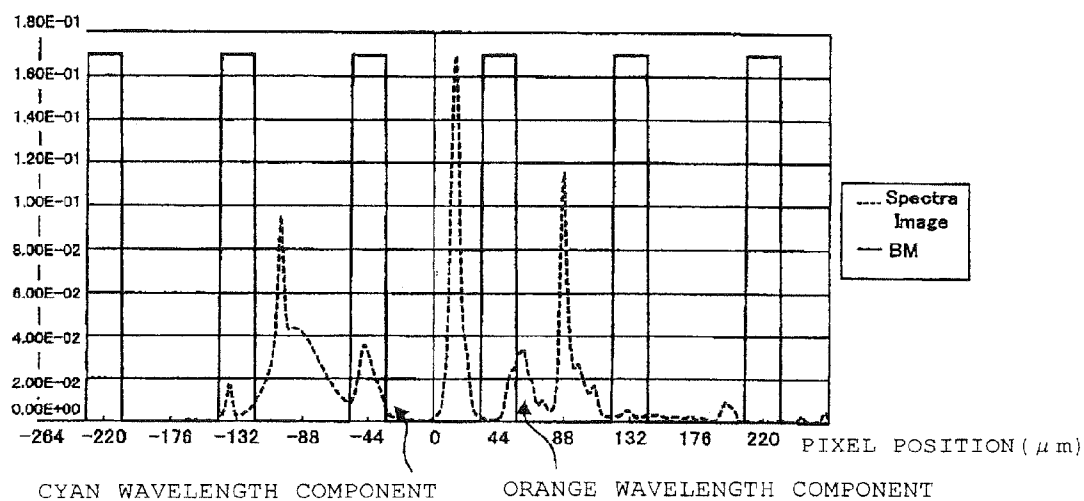
(a) POSITIONAL RELATIONSHIP BETWEEN CONVENTIONAL BM AND LIGHT SOURCE SPECTRUM
