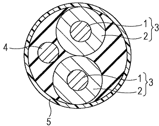
(b) SHIELD TWIST PAIR UNIT
