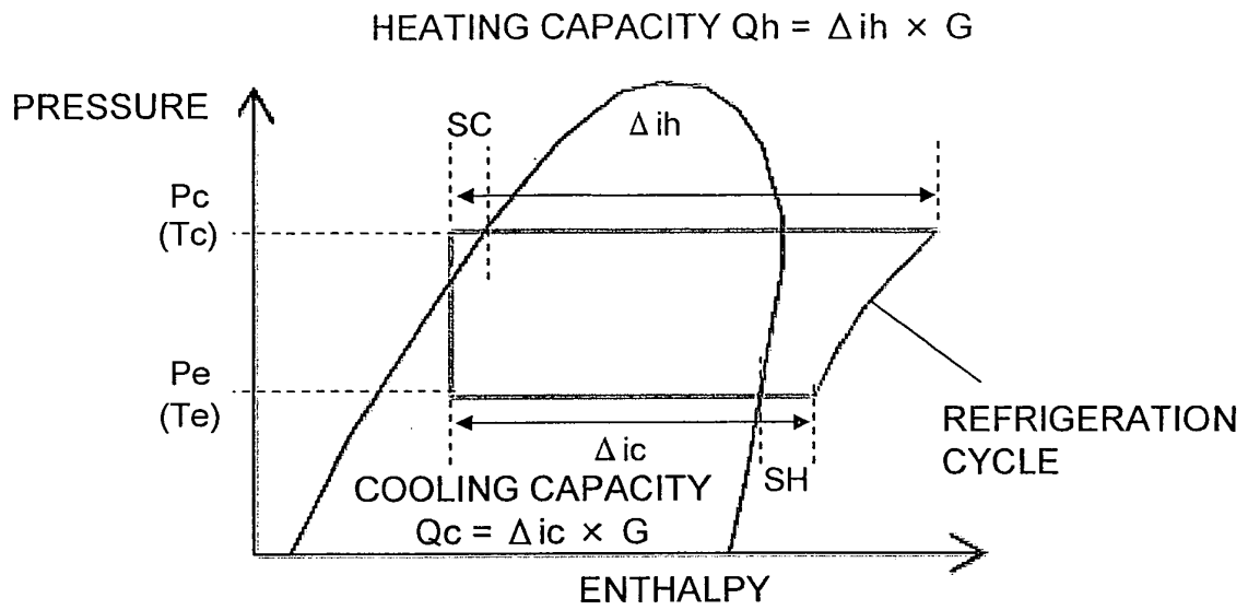
COOLING AND HEATING ENTHALPY DIFFERENCE (MOLLIER DIAGRAM)
