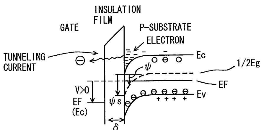
FIG. 30C PRIOR ART
