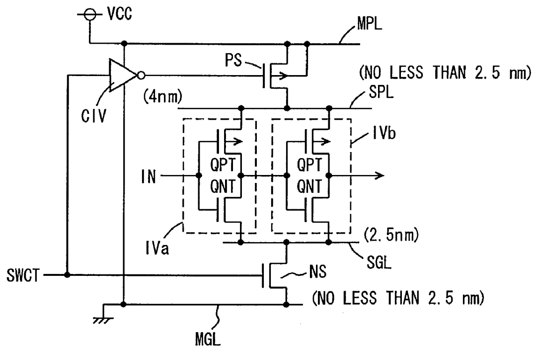
FIG. 31 PRIOR ART
