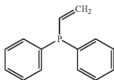
Diphenylvinylphosphine
