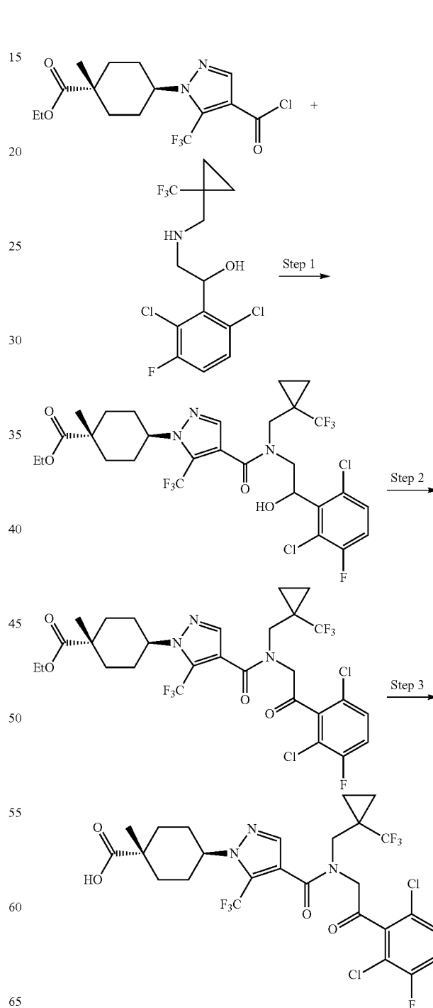
(1r,4r)-4-(4-((2-(2,6-dichloro-3-fluorophenyl)-2-oxoethyl)((1-(trifluoromethyl)cyclopropyl)methyl)carbamoyl)-5-(trifluoromethyl)-1H-pyrazol-1-yl)-1-methylcyclohexanecarboxylic acid
