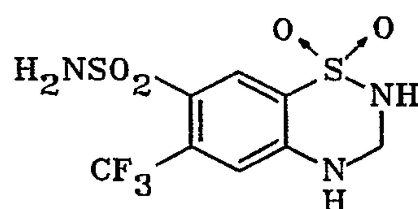
33 hydroflumethiazide
