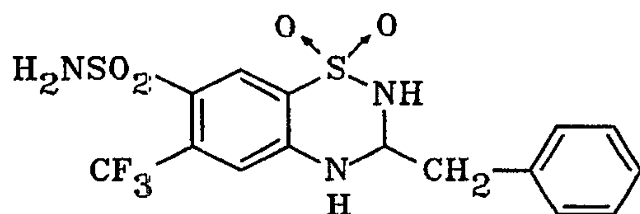
26 bendroflumethiazide
