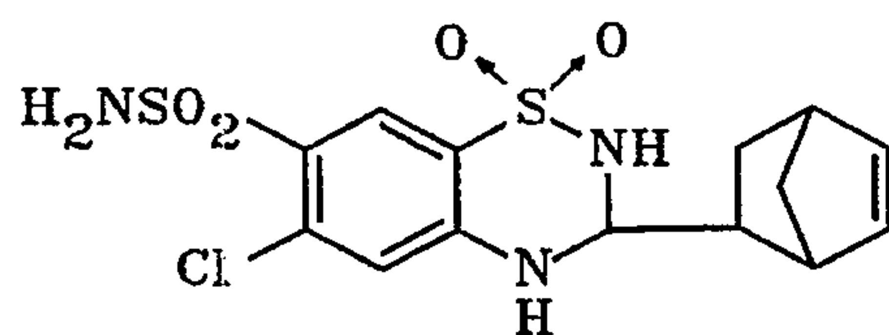
30 cyclothiazide
