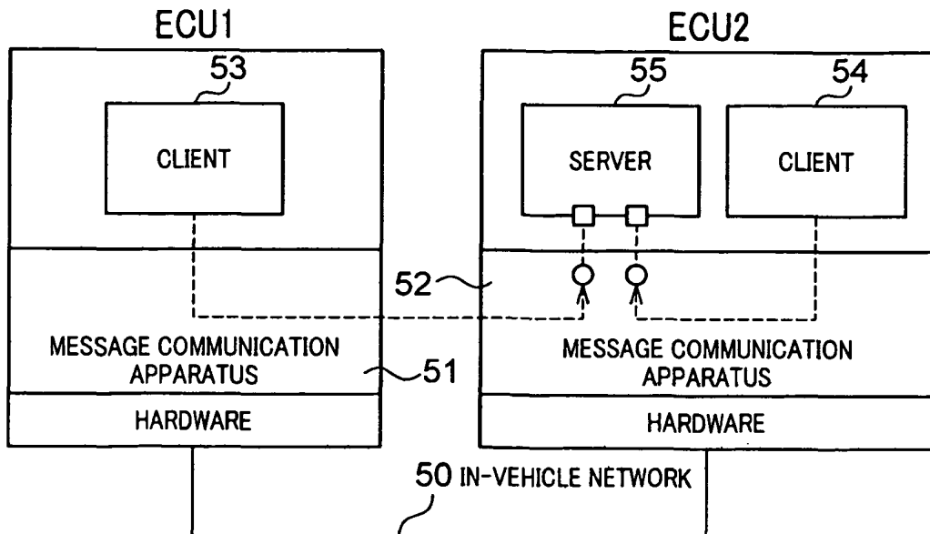
FIG. 10 PRIOR ART
