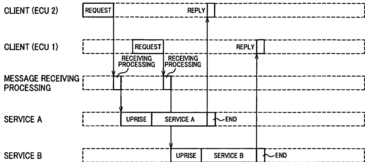
FIG.11 PRIOR ART
