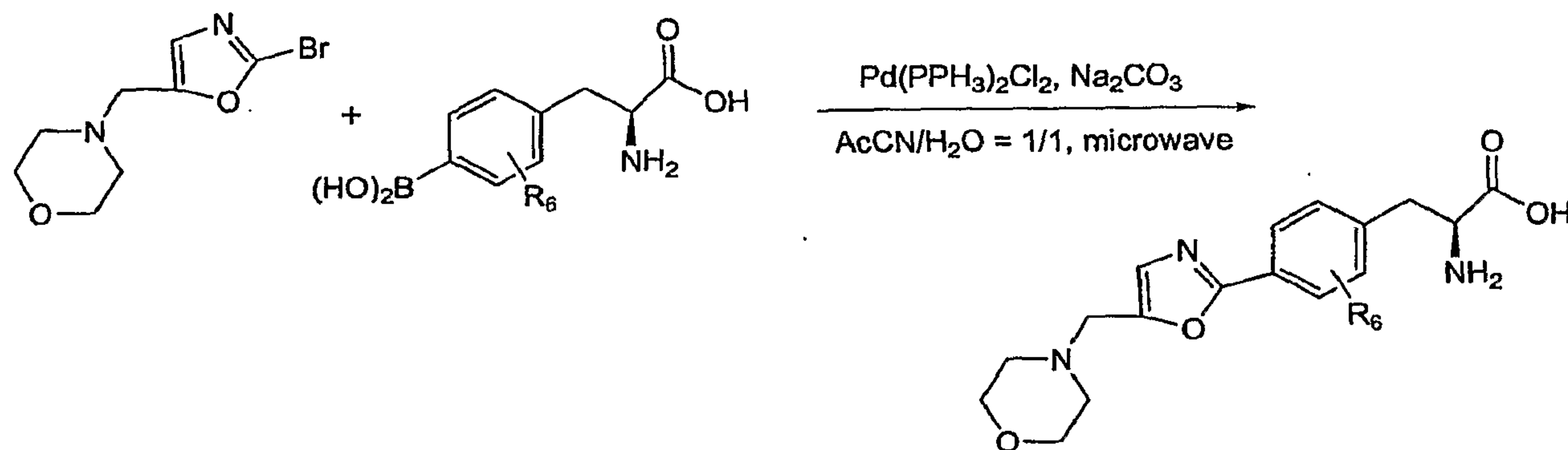
Scheme 7
