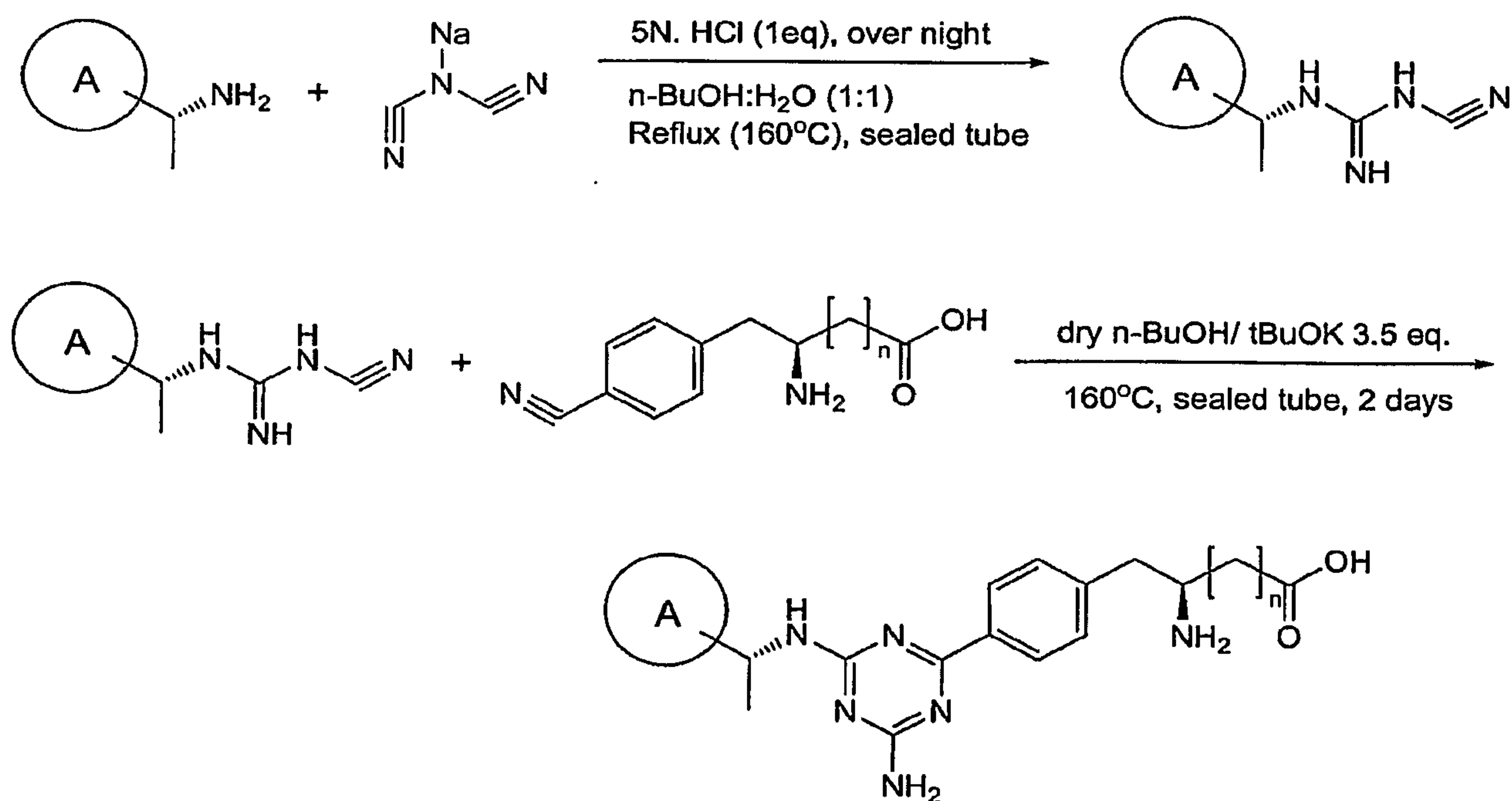
Scheme 6
