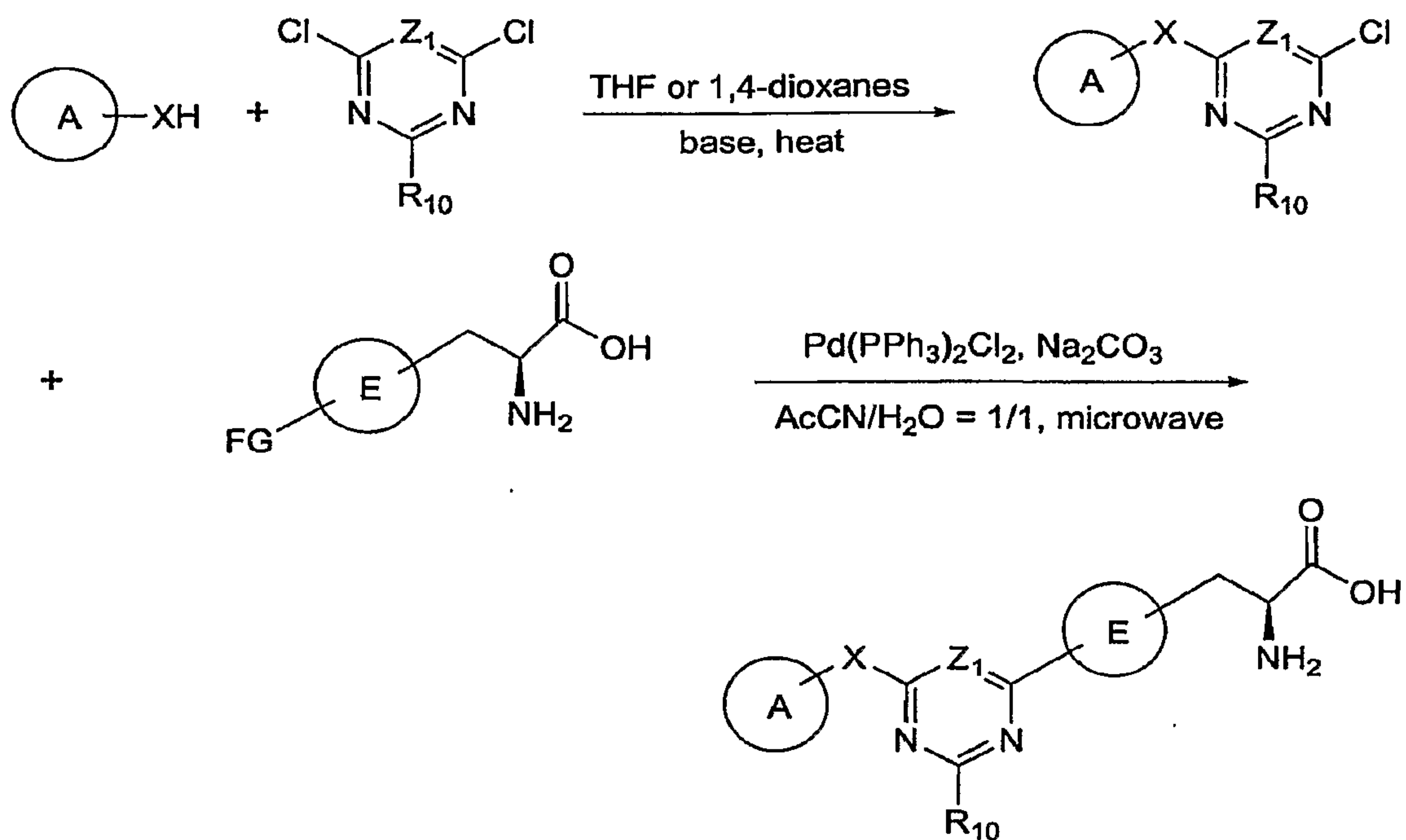
Scheme 4
