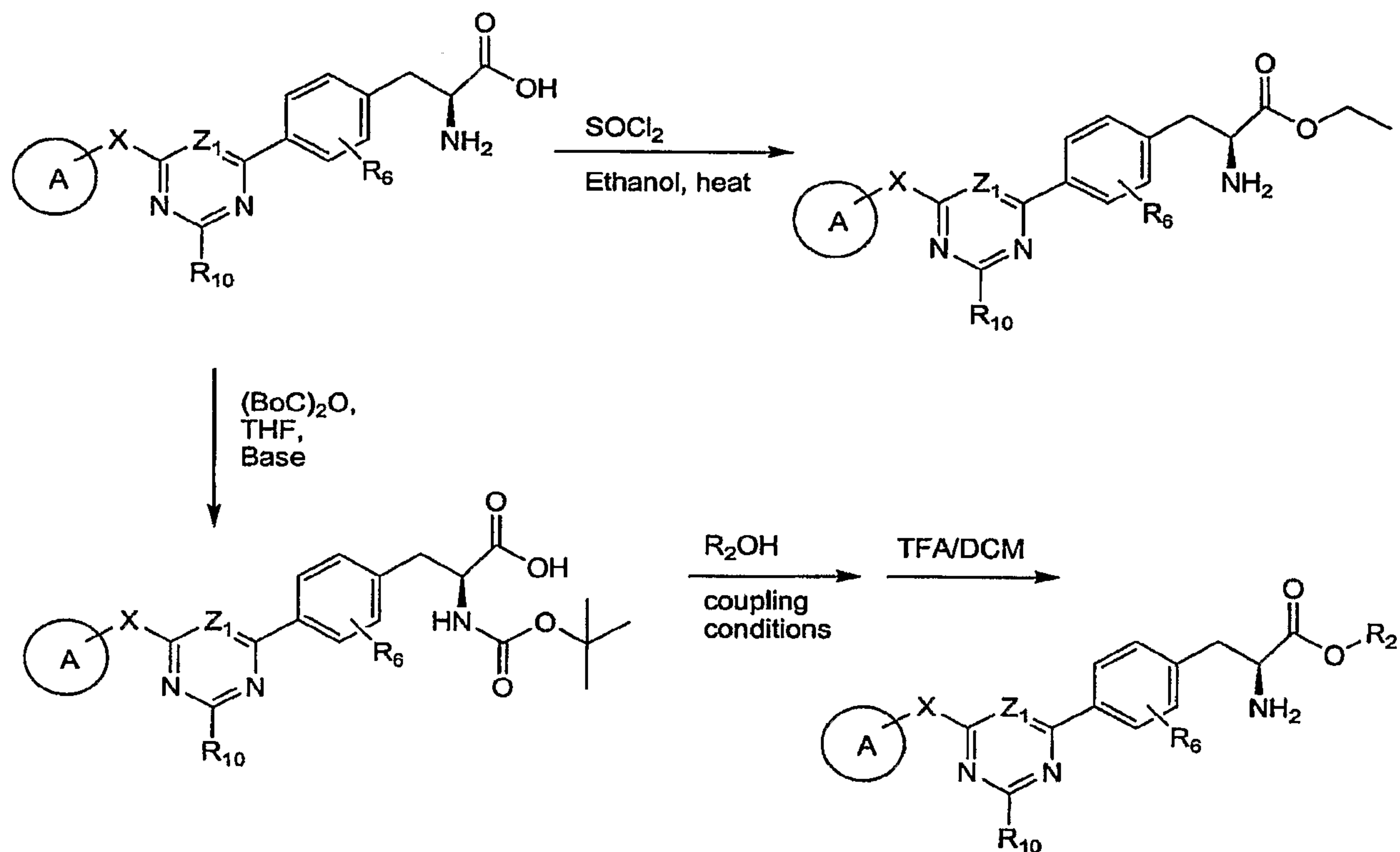
Scheme 5
