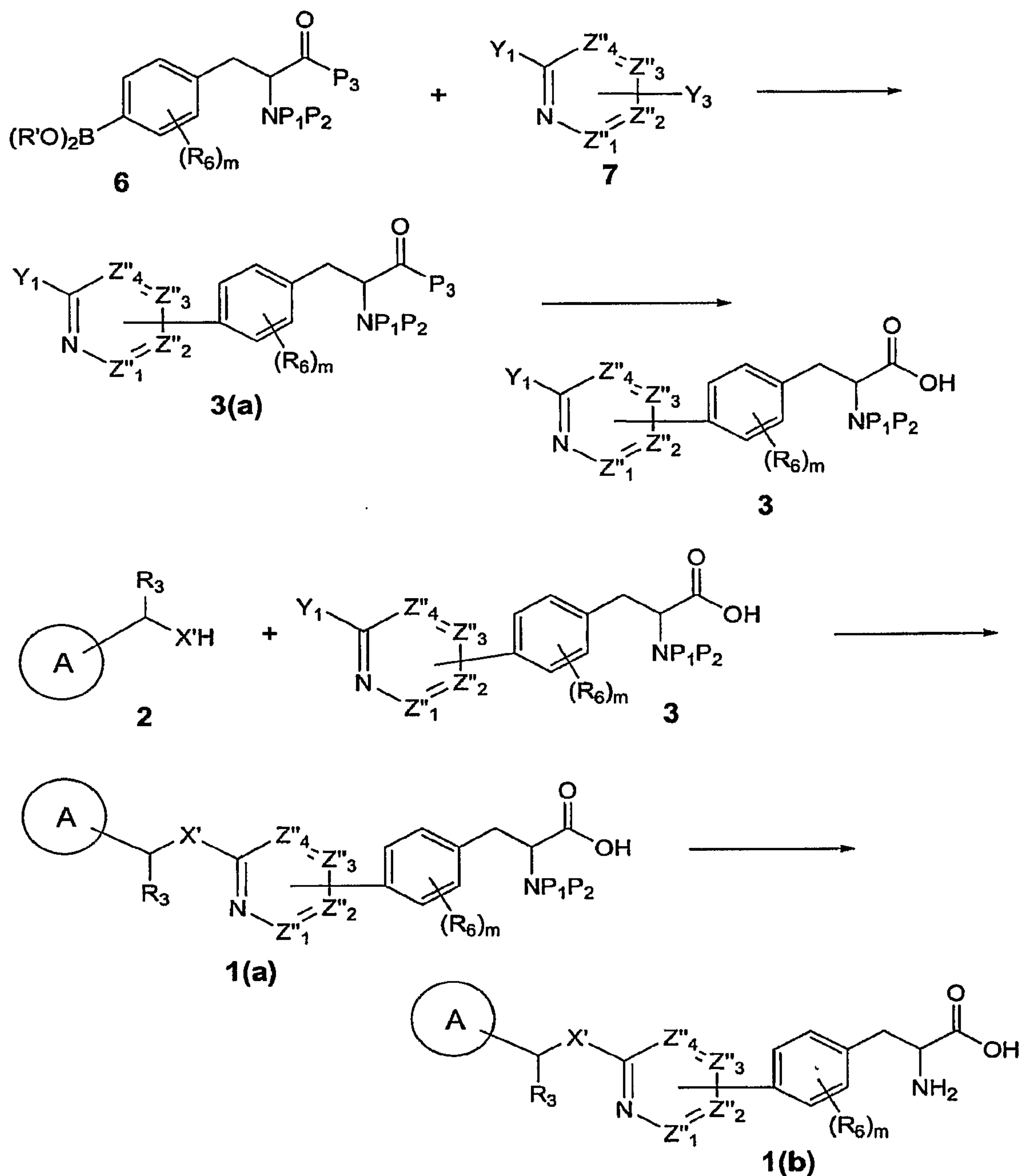
Scheme 3
