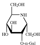
5-O-α-D-Galactopyranosyl-α-homonojirimycin
