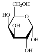
α-D-Galactose
