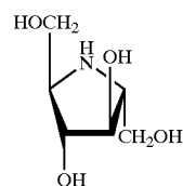
2,5-Dideoxy-2,5-imino-D-mannitol
