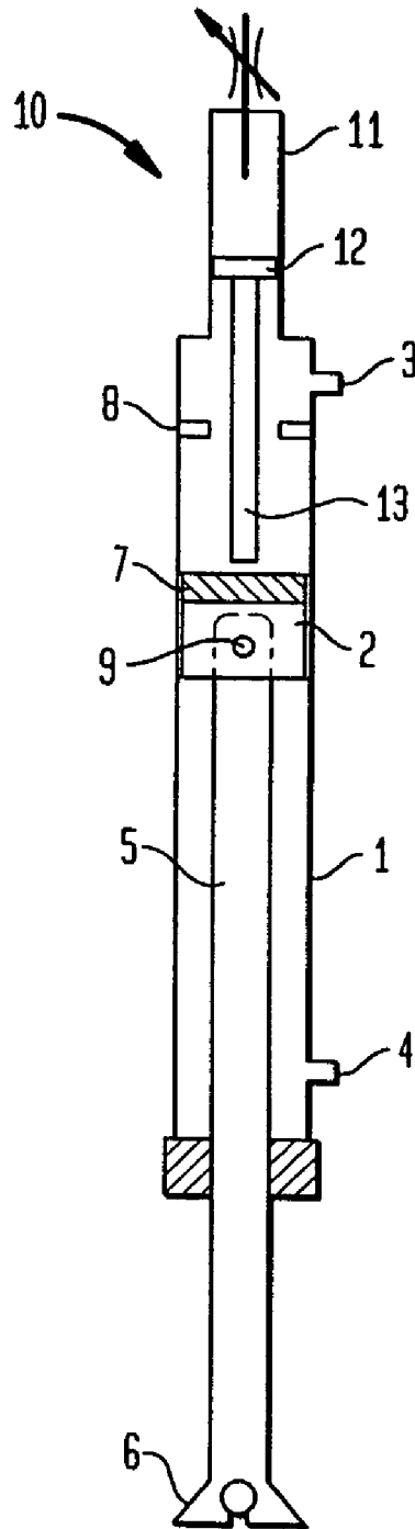
FIG. 5 (PRIOR ART)
