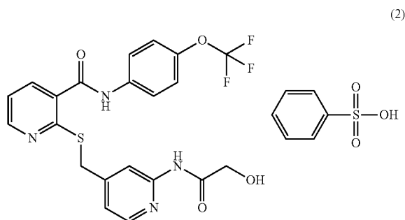
[Chemical 2]
