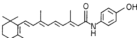
N-(4-HYDROXYPHENYL) RETINAMIDE
