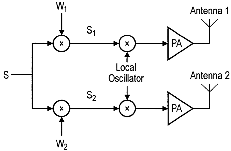
High level implementation of UE uplink transmit diversity
