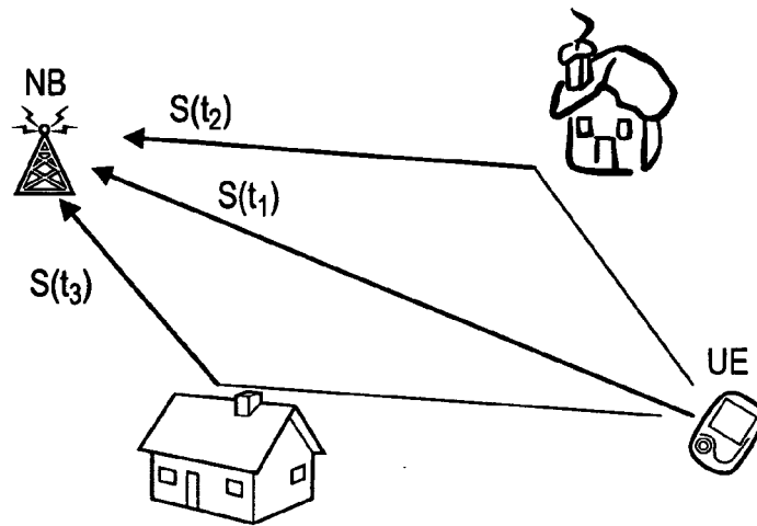
Multipath propagation
