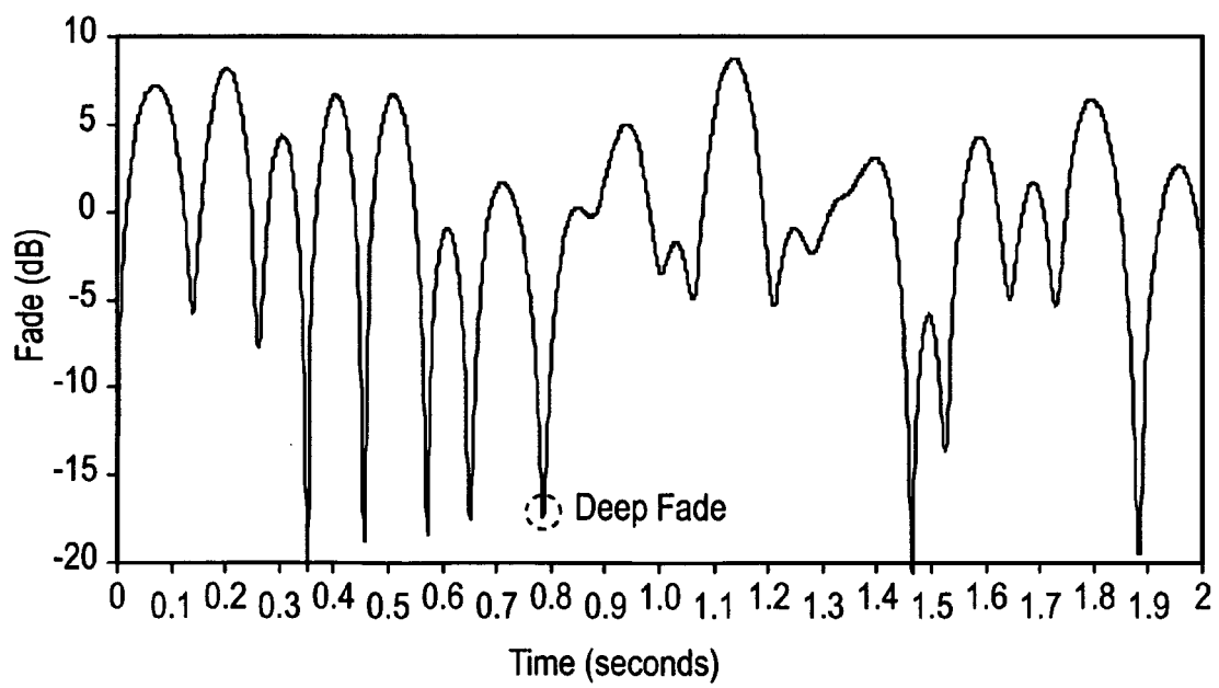
Fast fading in time for a UE moving at 3 kmph
