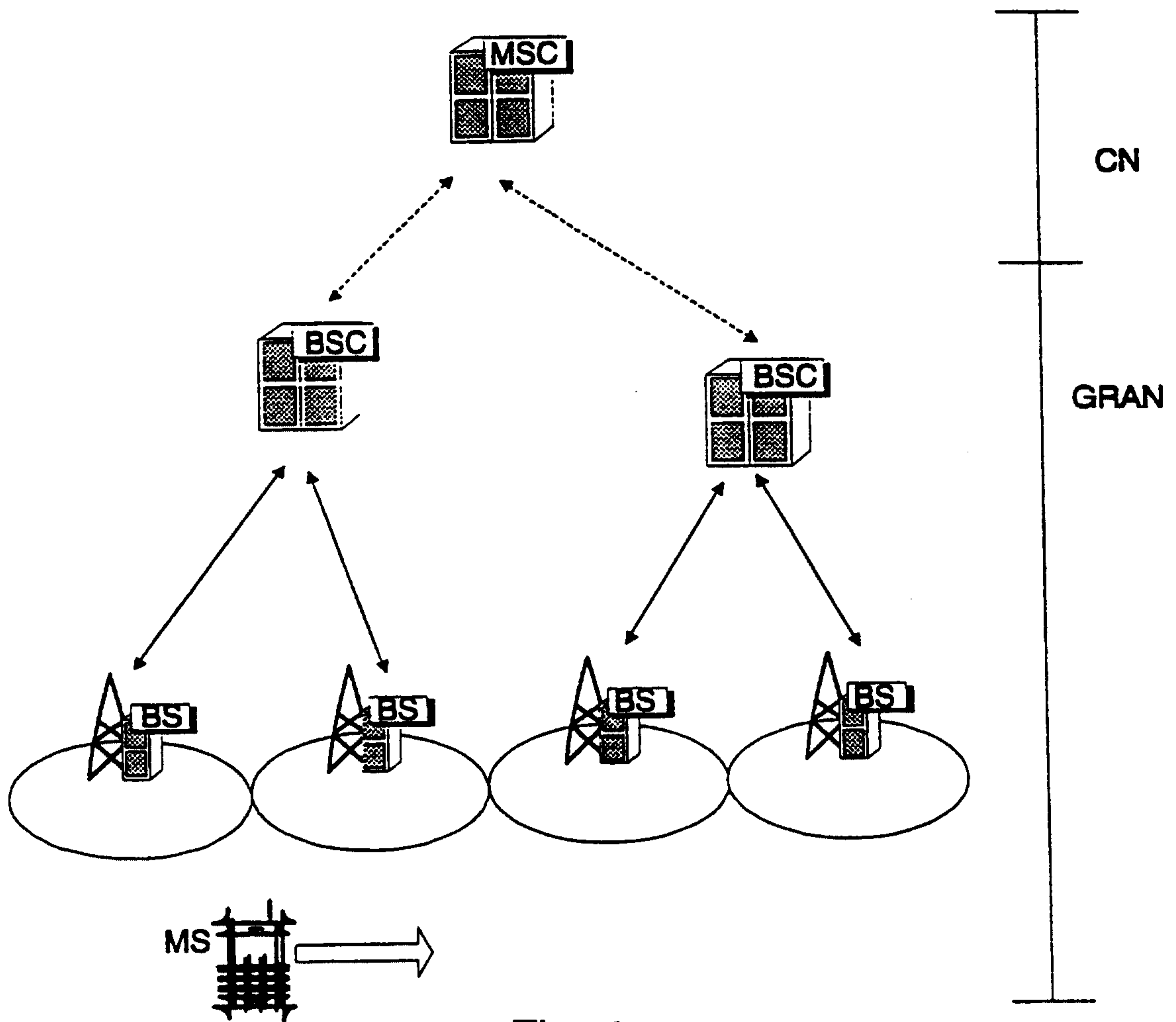
Fig. 4 PRIOR ART
