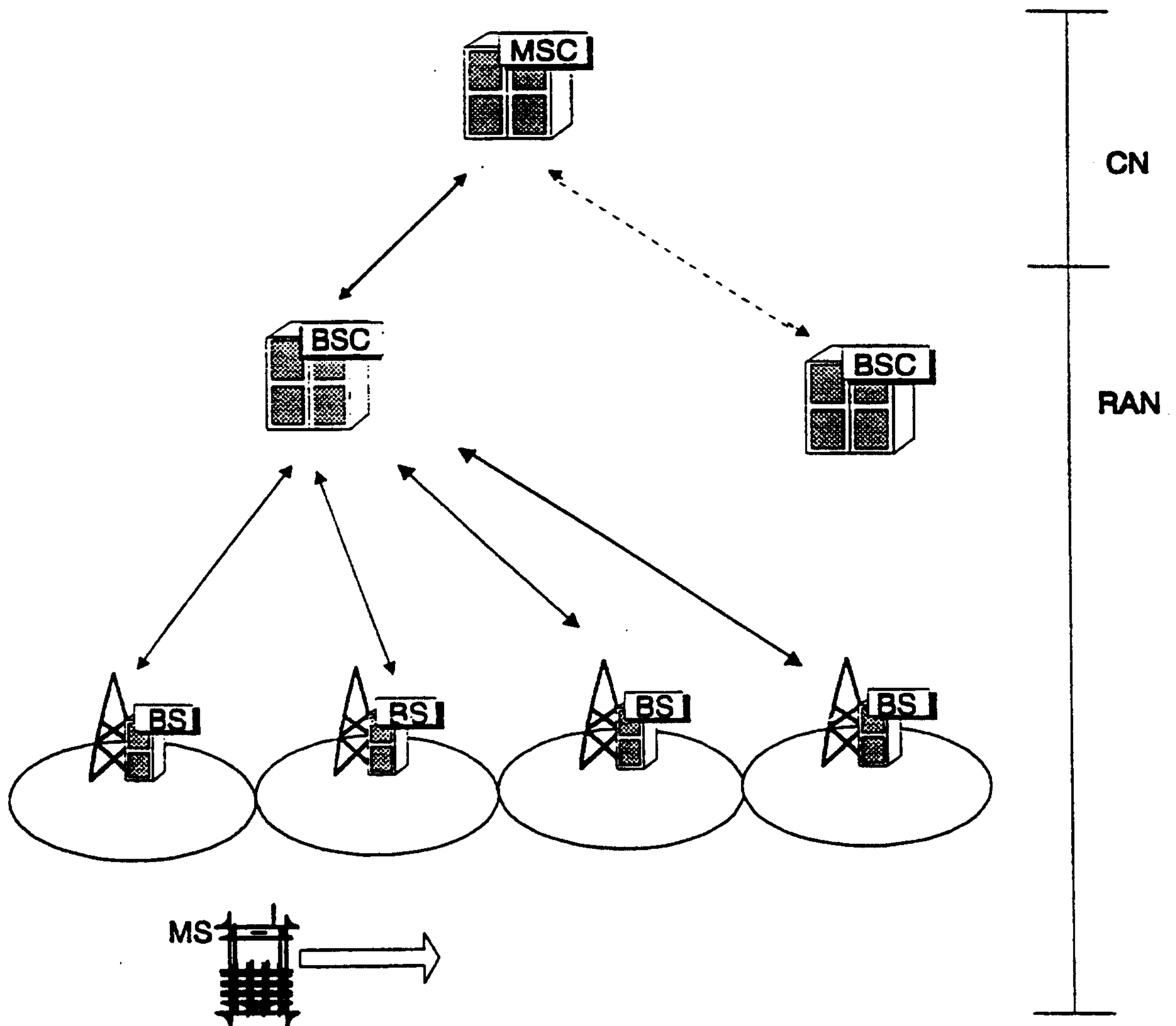
Fig. 1 PRIOR ART
