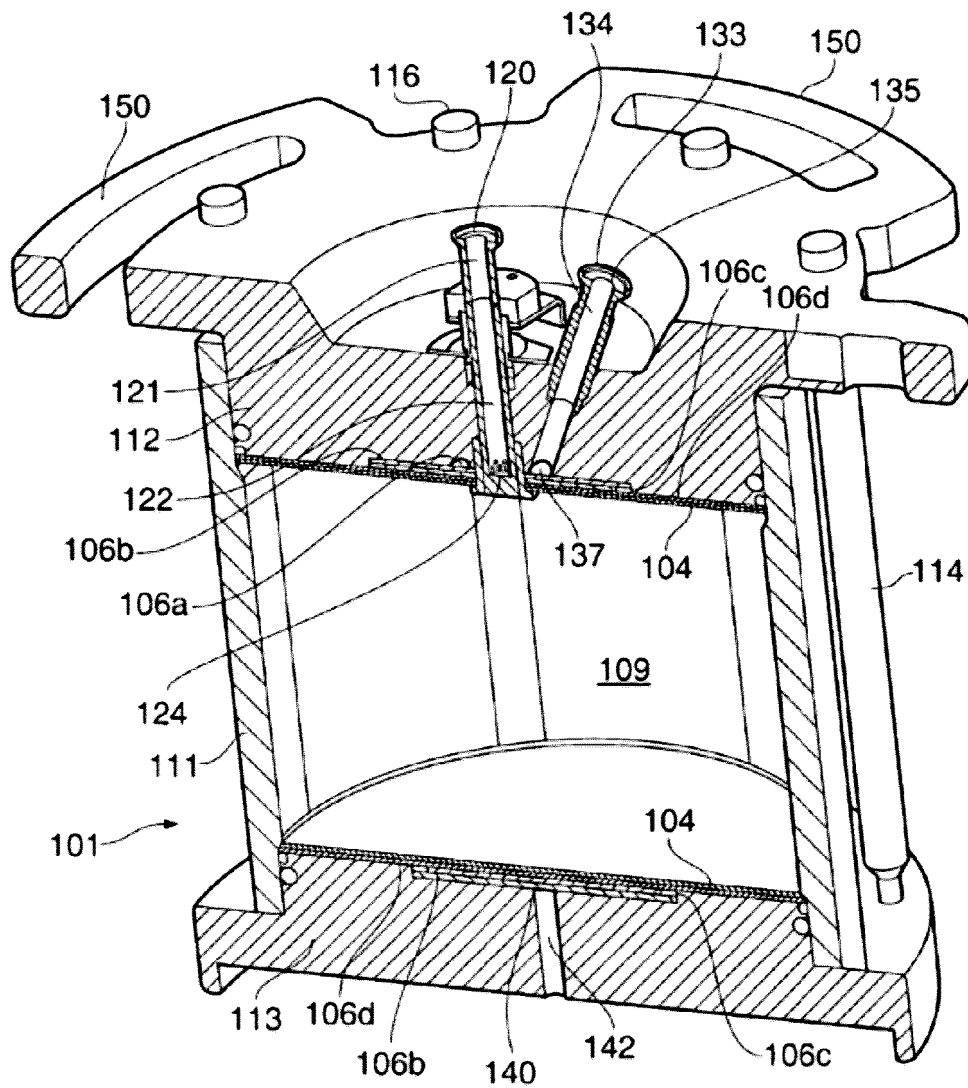
Figure 1 – PRIOR ART
