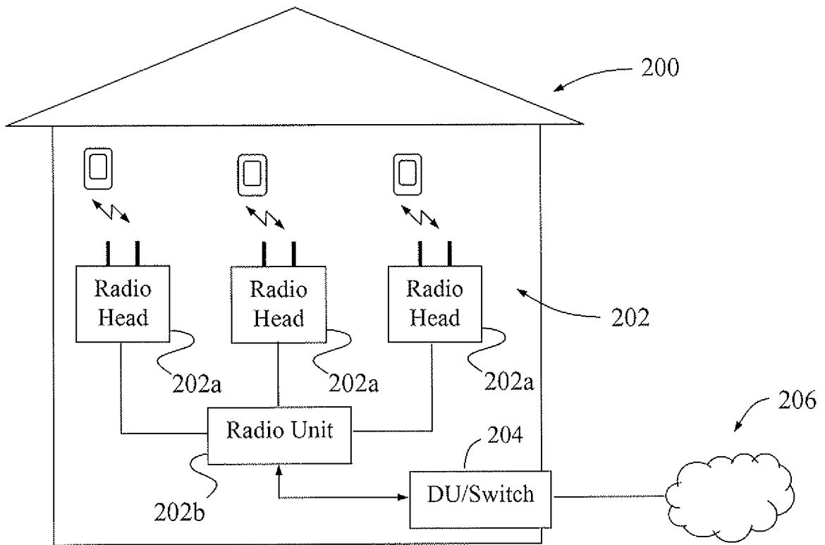
Fig. 2 (Prior art)
