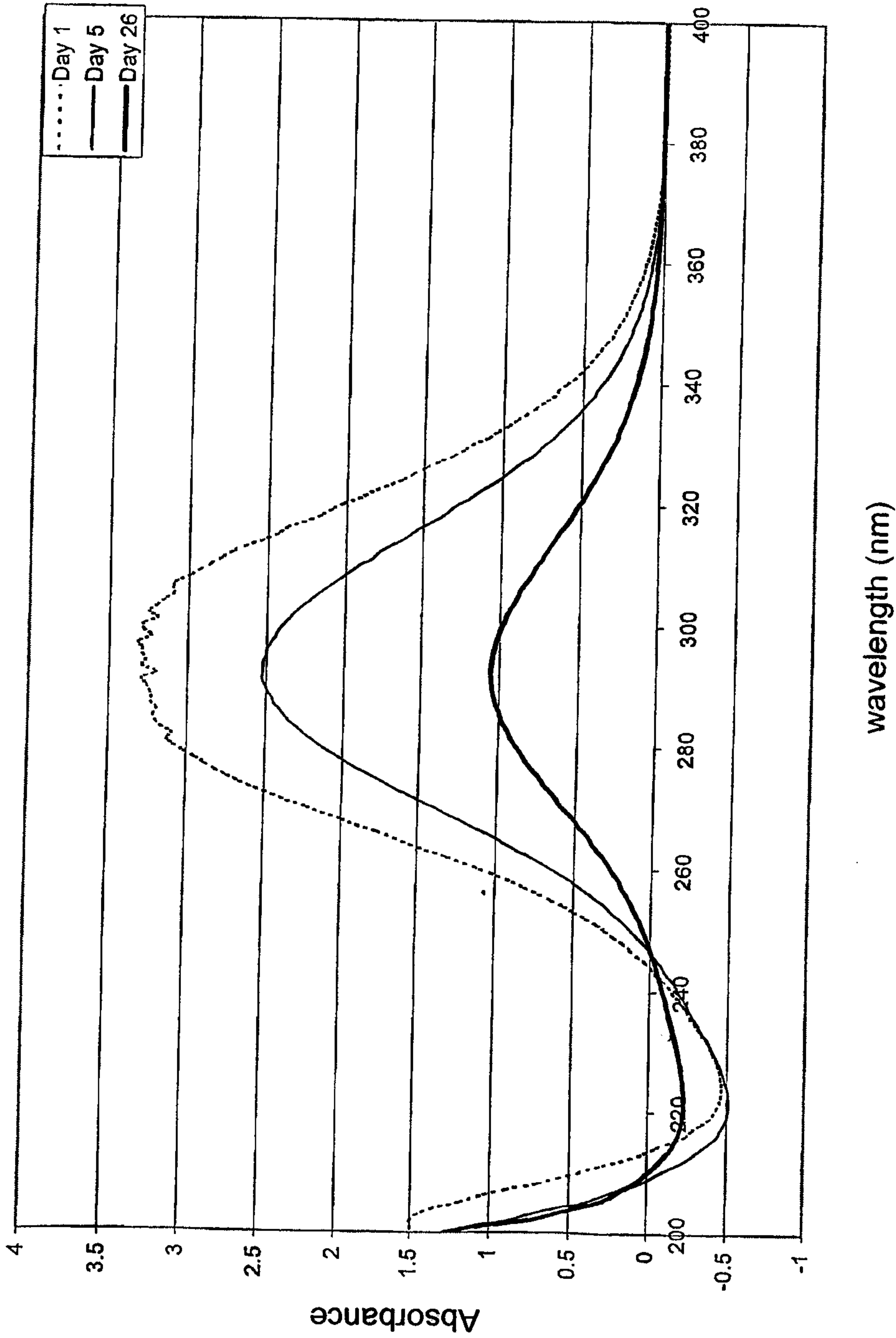
Fig. 3: Spectrophotometer Readings 2500 ppm Hydrogen Peroxide: 25000 ppm Sodium Hypochlorite Mixture Baseline 2500 ppm Hydrogen Peroxide
