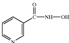
nicotinuric acid:
