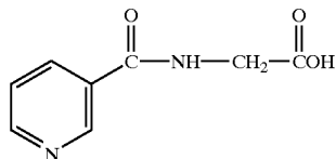
nicotinuric acid:
