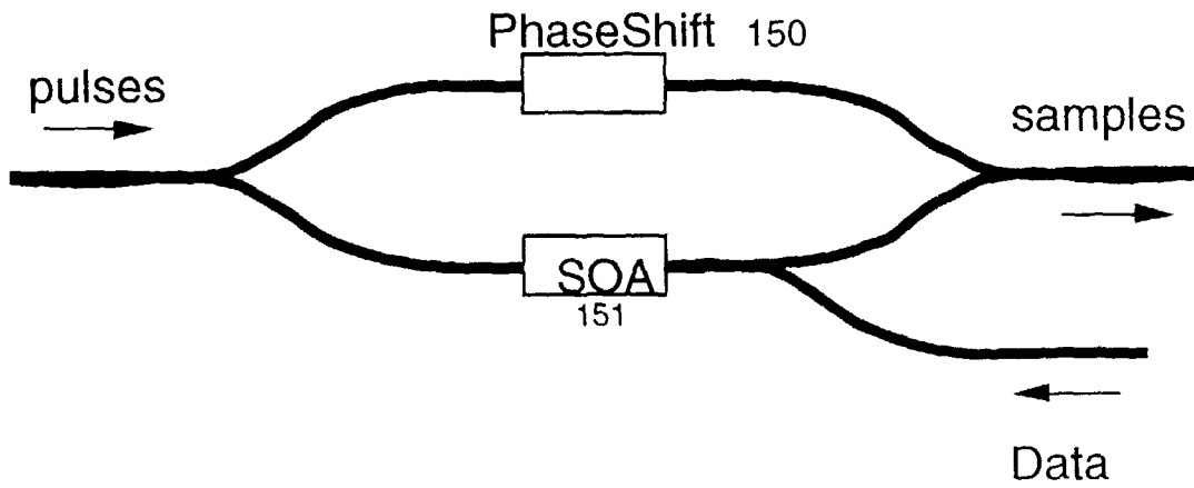
Fig 19 Interferometer Arrangement
