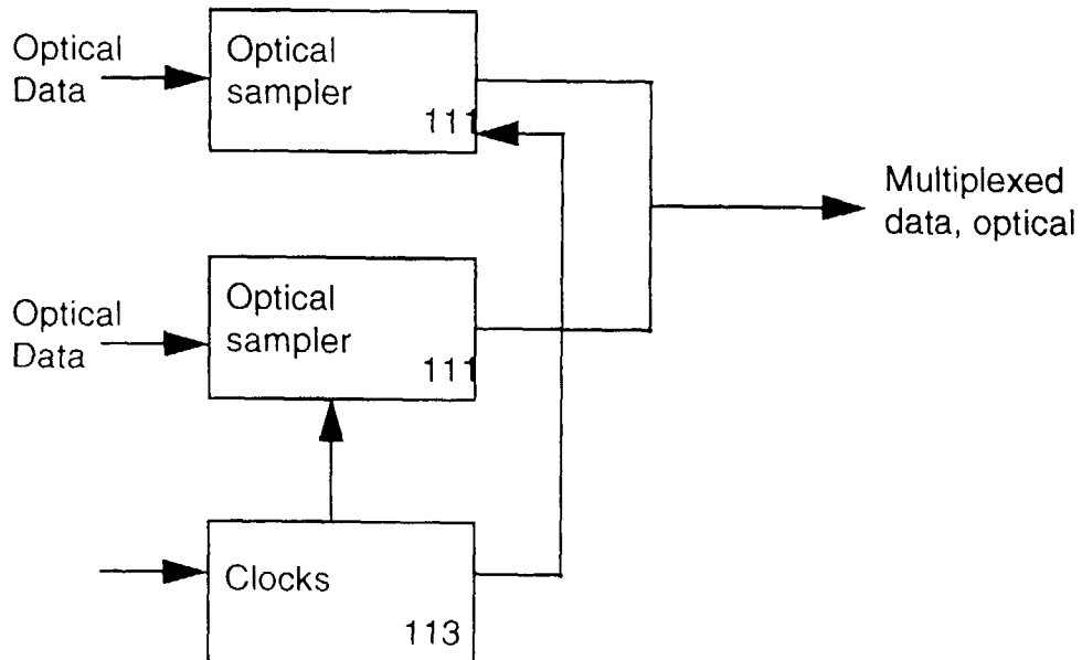
Fig 14 MULTIPLEXER
