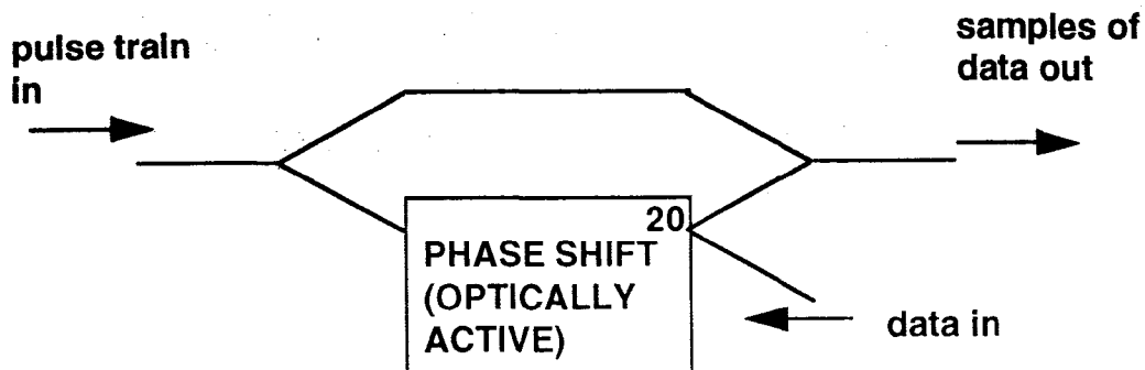
Fig 3 INTERFEROMETER ARRANGEMENT
