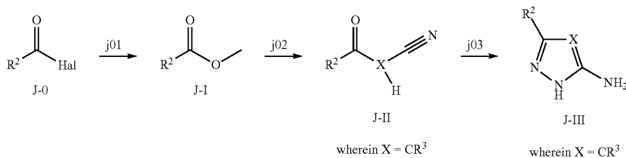
General reaction scheme (scheme 1a):
