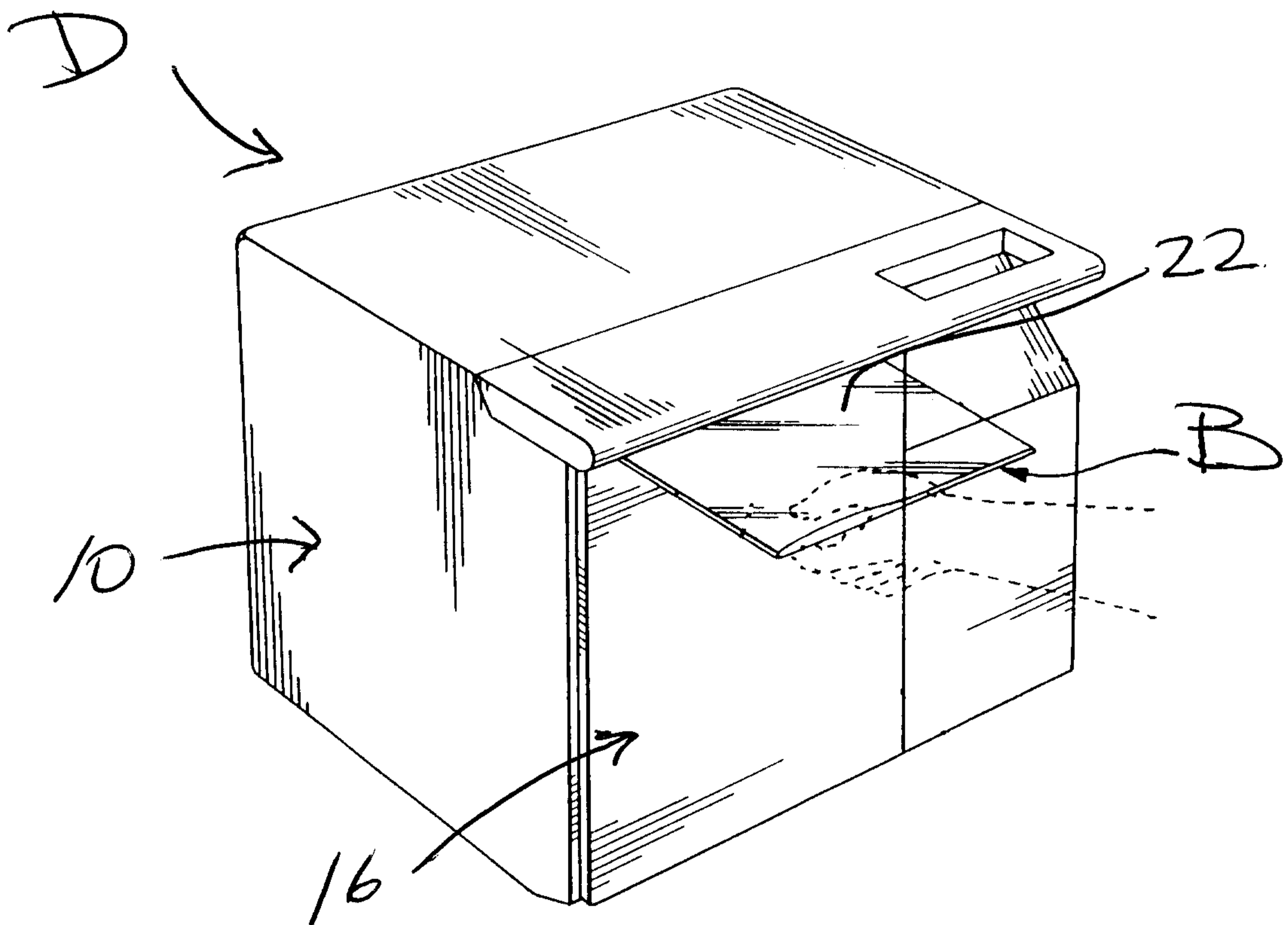
FIG. 2 (PRIOR ART)
