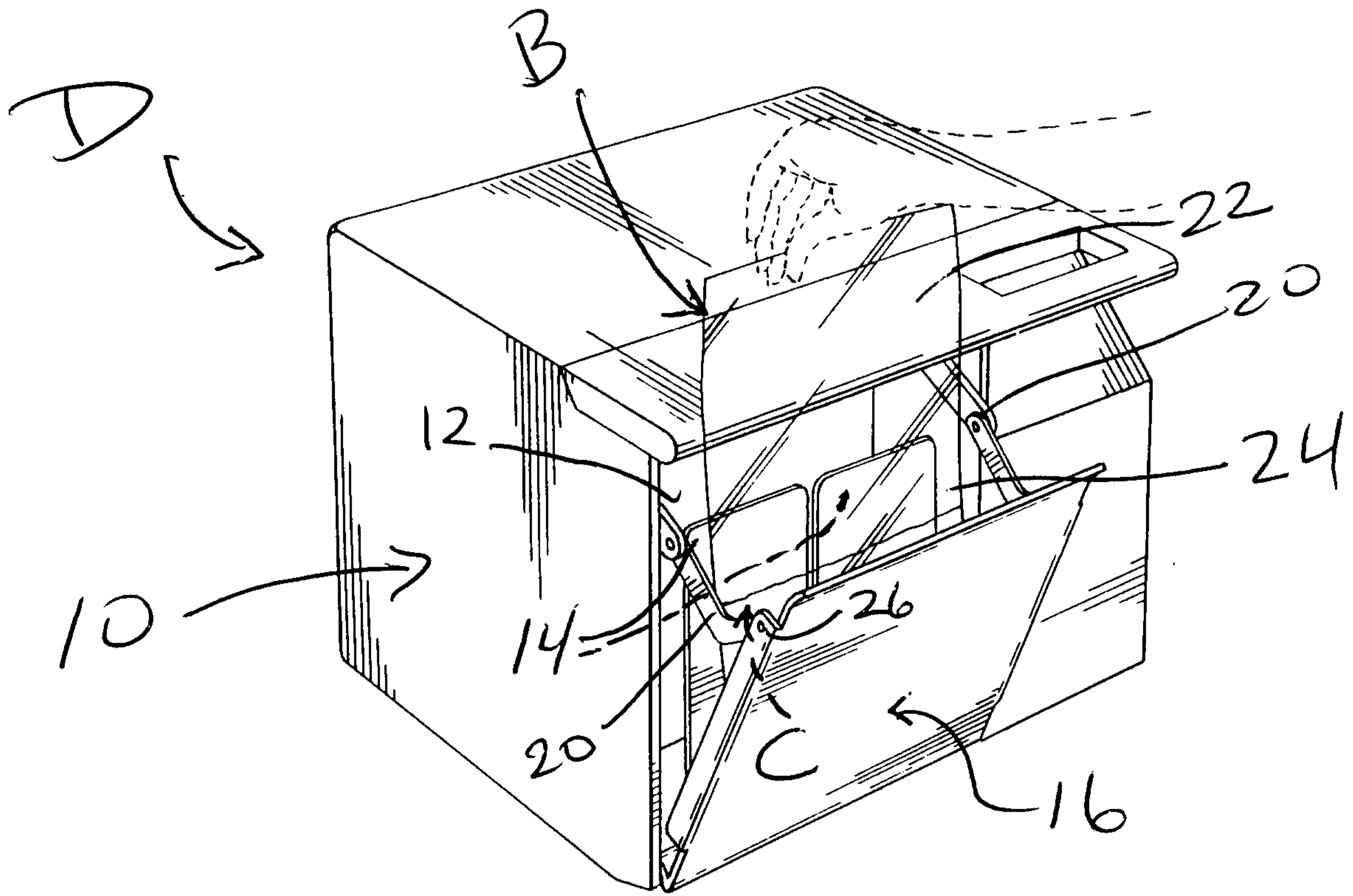
FIG. 1 (PRIOR ART)
