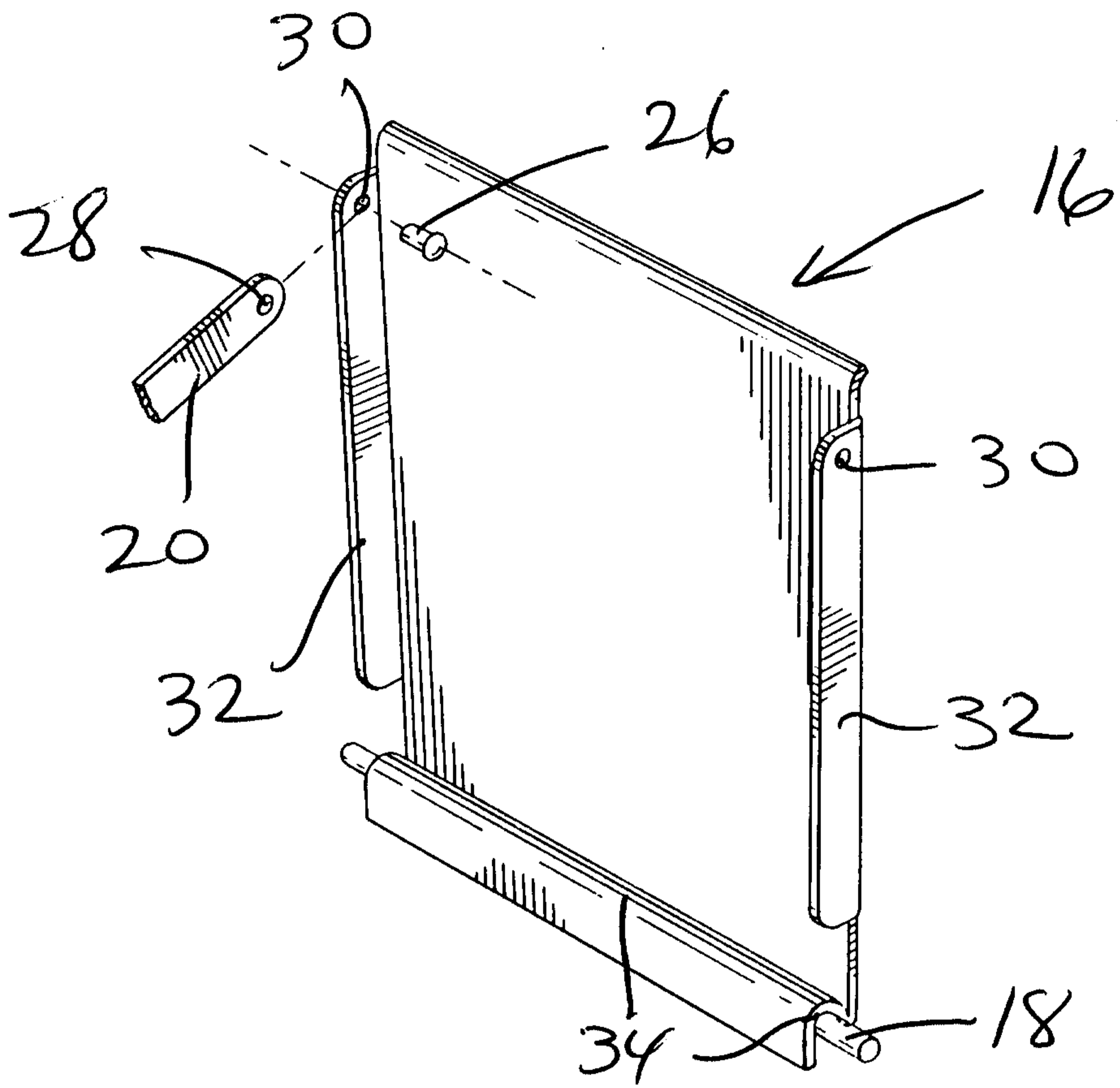
FIG. 3 (PRIOR ART)
