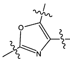
2-AMINO-5-ARYL-OXAZOLE
