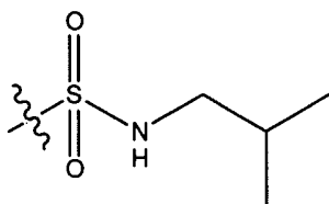
isobutylsulfonamide
