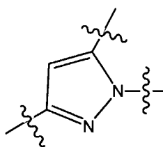
3-AMINO-PYRAZOLE
