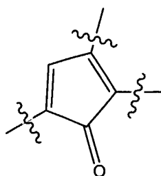
CYCLOPENTADIENONE
