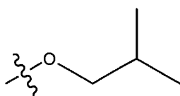
isobutoxy
