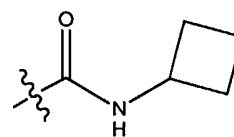
cyclobutylamide
