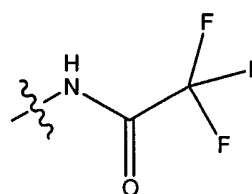
aminoacyltrifluoromethyl
