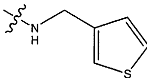
3-aminomethylthiophene
