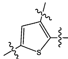
THIOPHENE
