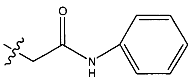
benzylacetylamine
