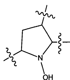
N-HYDROXYPYRROLIDINE
