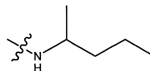
sec-pentylamine
