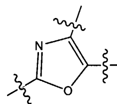
2-AMINO-4-ARYL-OXAZOLE
