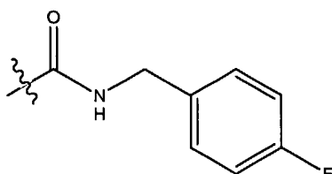
p-fluorobenzylamide
