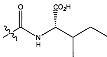
1-carboxyl-2-methylbutylamine
