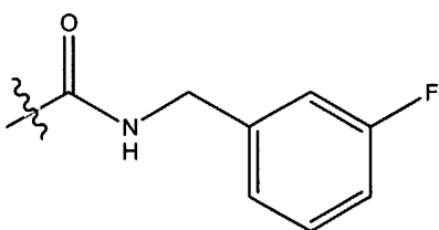
m-fluorobenzylamide
