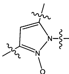
PYRAZOLE-N-OXIDE
