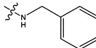
benzylamine
