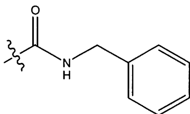
carboxamidobenzyl
