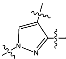
1-AMINO-PYRAZOLE
