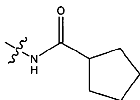
cyclopentylacetylamine
