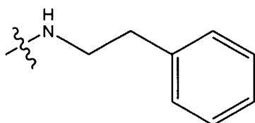
phenethylamine
