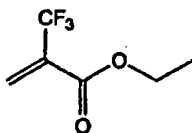
[Chem. 8]
