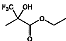
[Chem. 7]
