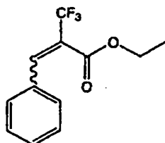
[Chem. 15]
