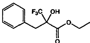
[Chem. 16]
