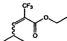
[Chem. 24]
