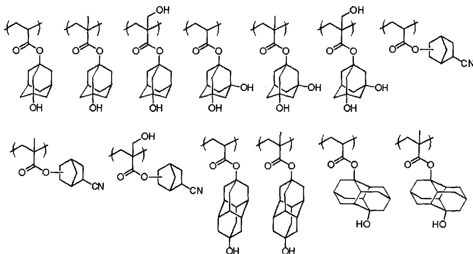
[Chem. 21]
