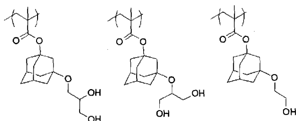
[Chem. 21]
