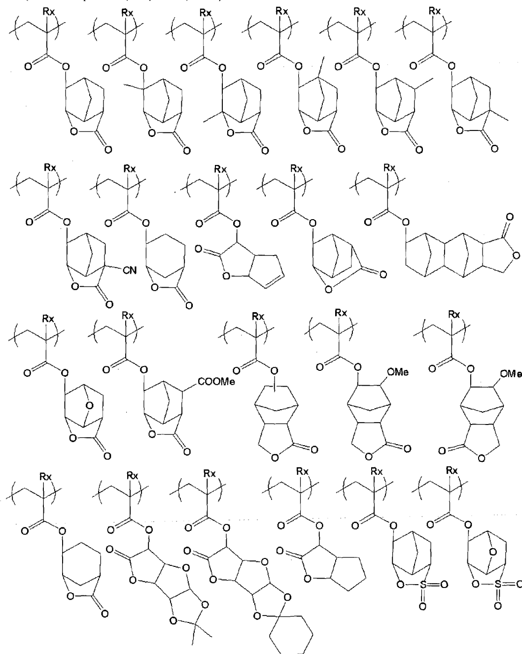
[Chem. 15]
