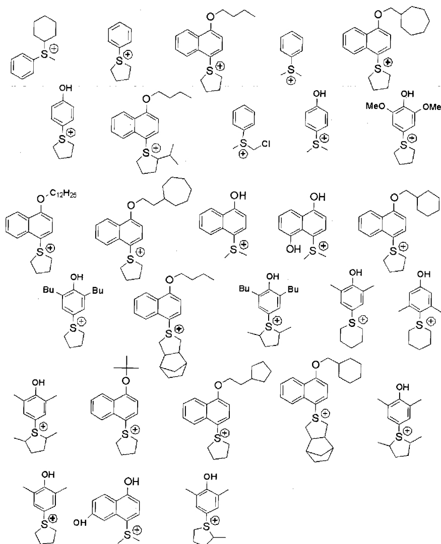
[Chem. 43]
