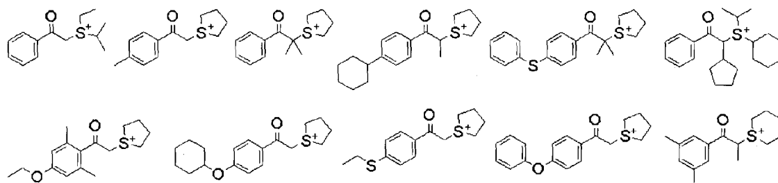
[Chem. 40]
