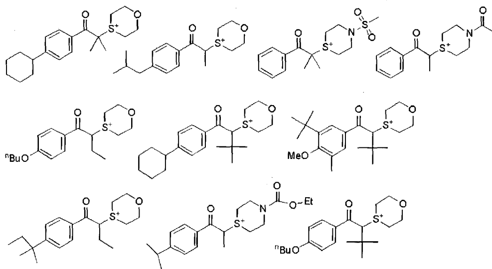
[Chem. 40]
