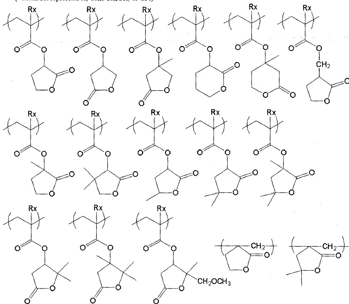
[Chem. 14]
