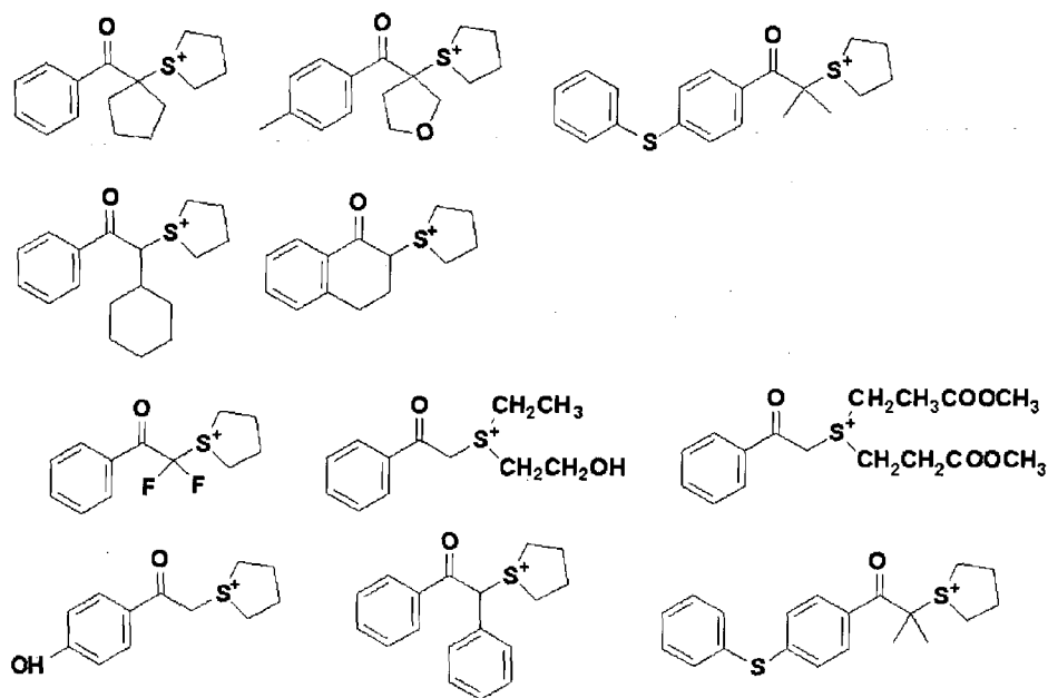
[Chem. 39]
