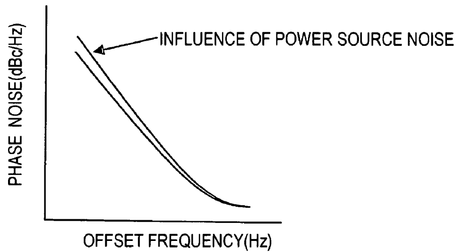
FIG. 4 (PRIOR ART)
