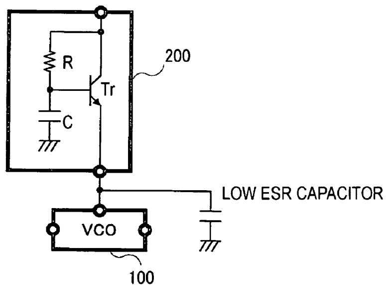
FIG. 5 (PRIOR ART)
