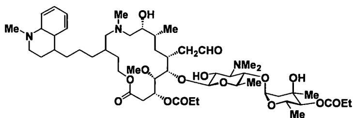
Example 60 (Stereoisomer of the compound of Example 54)
