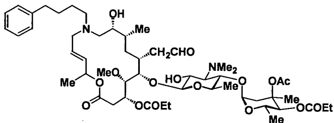
Example 47 (Stereoisomer of the compound of Example 46)
