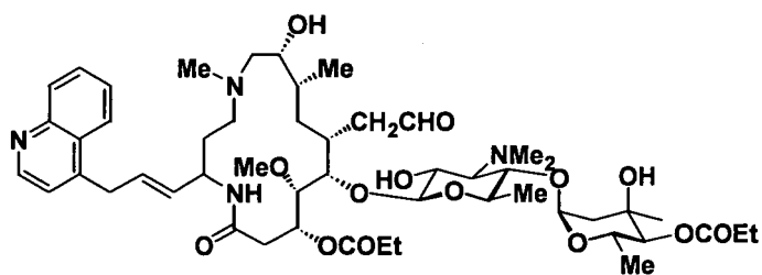
Example 29 (Stereoisomer of the compound of Example 28)
