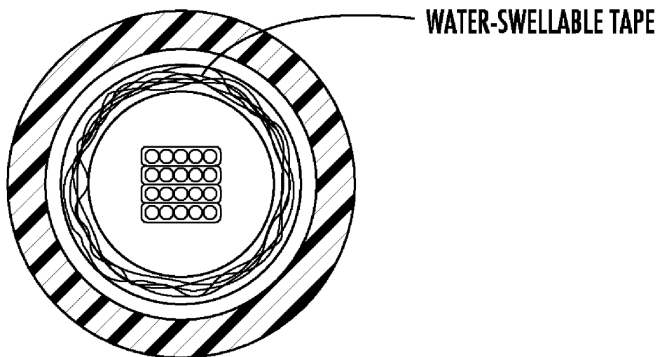
FIG. 12 (PRIOR ART)
