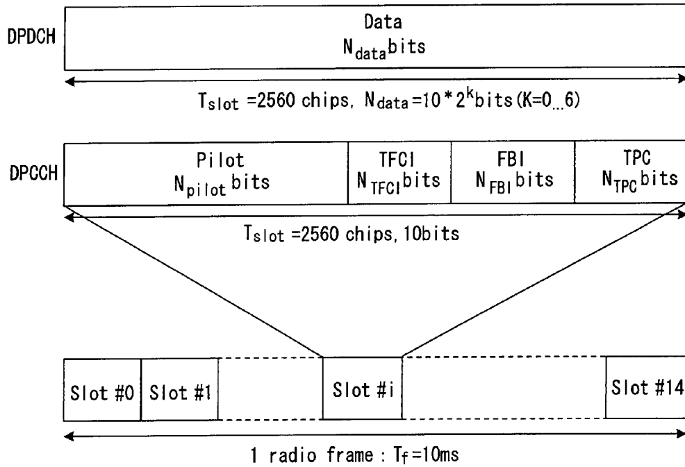
FIG. 9 PRIOR ART
