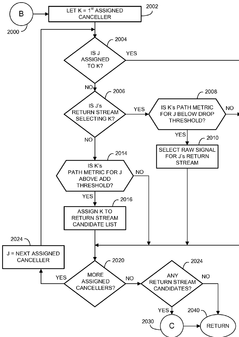
Figure 20 RS Control Algorithm – Create RS Candidate List
