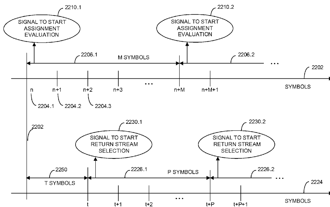
Figure 22 Scheduler for Execution Signals
