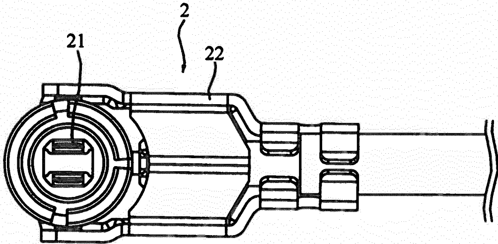
Figure 2(Prior Art)
