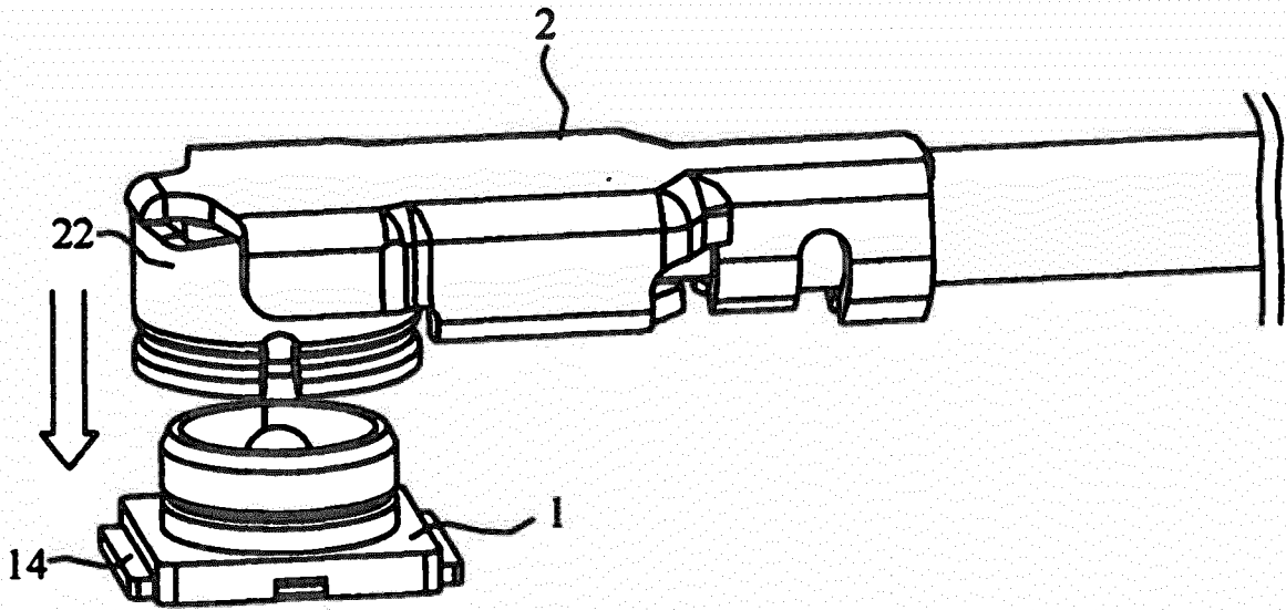
Figure 3(Prior Art)
