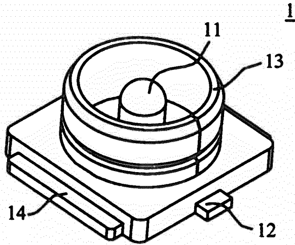
Figure 1(Prior Art)
