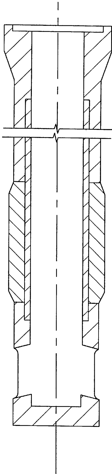
FIG. 19 PRIOR ART
