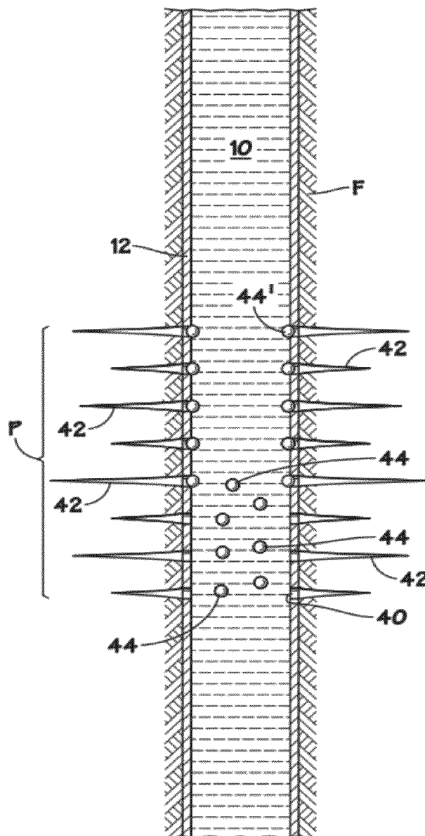
FIG. 6 (PRIOR ART)
