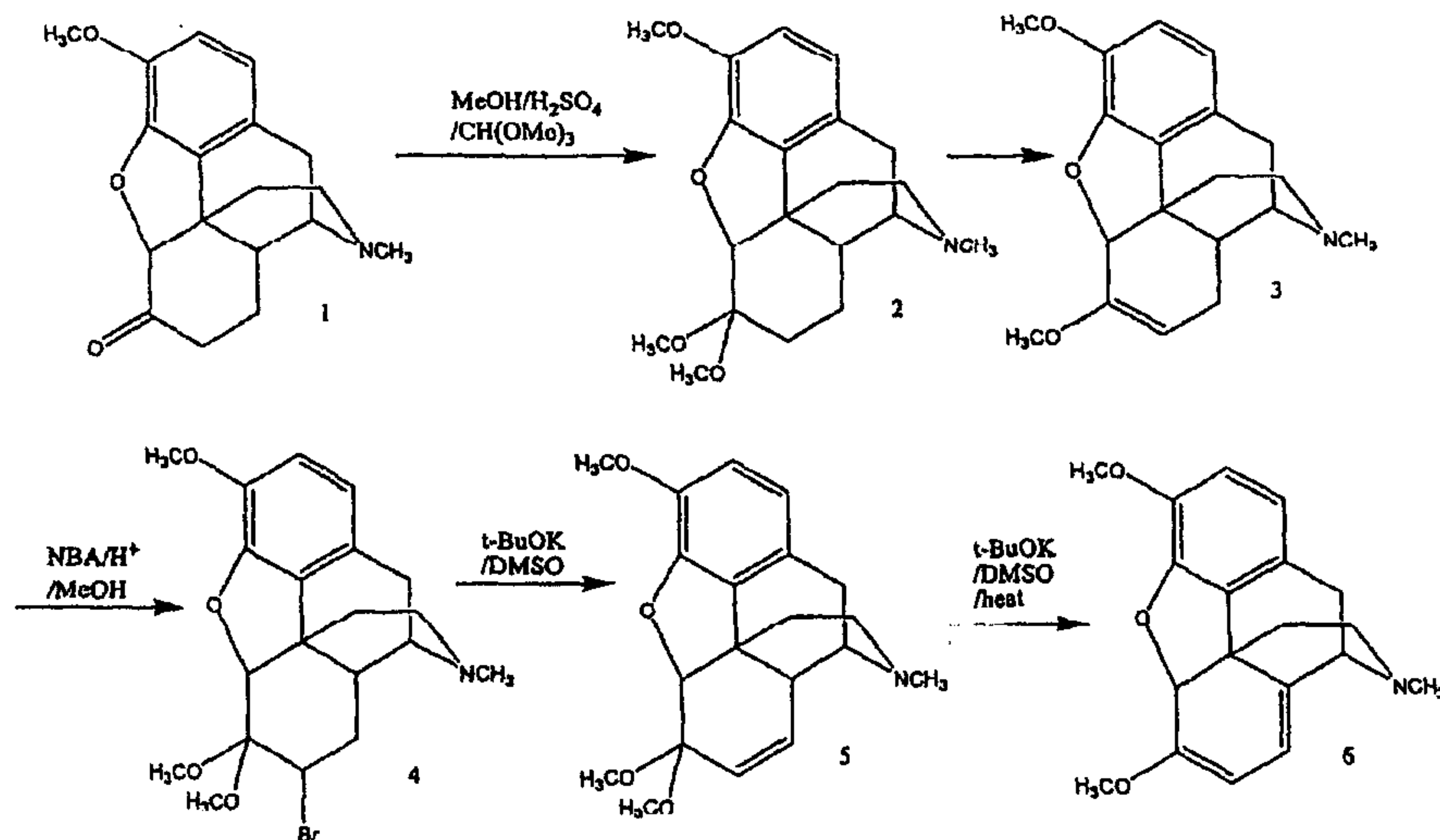
Conventional Route for making thebaine Scheme 1
