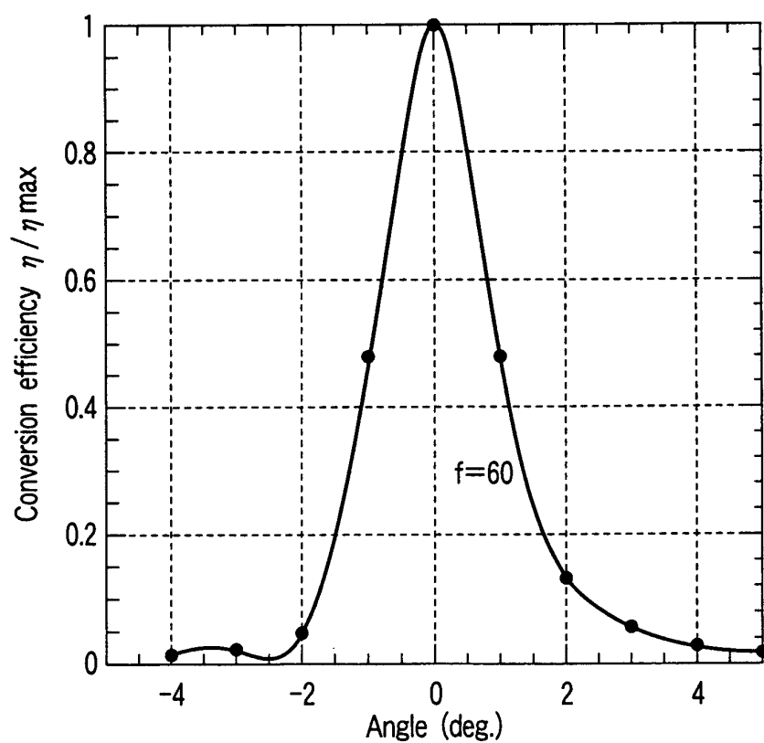
FIG. 13 Elevation angle dependency of SHG conversion efficiency
